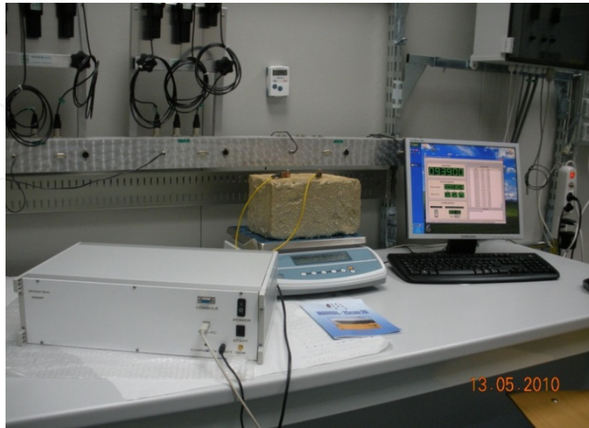
Figure 4. Experimental set up.
