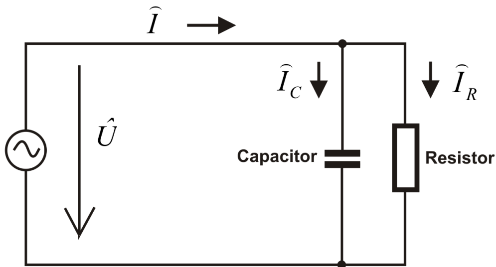
Figure 1. Equivalent diagram of measured impedance.
