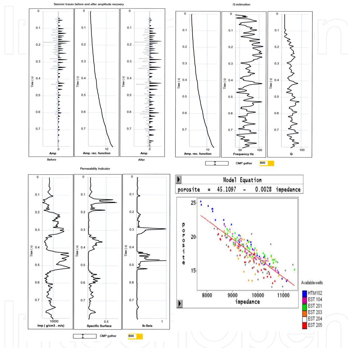
Figure 6. Seismic analysis at CMP 600. [4] Top from left to right: seismic trace before and after amplitude recovery, amplitude recovery function, instantaneous frequency trace and Q seismic trace. Bottom from left to right: acoustic impedance trace, Specific surface and Ik-Seis traces, porosity – acoustic impedance relationship.
