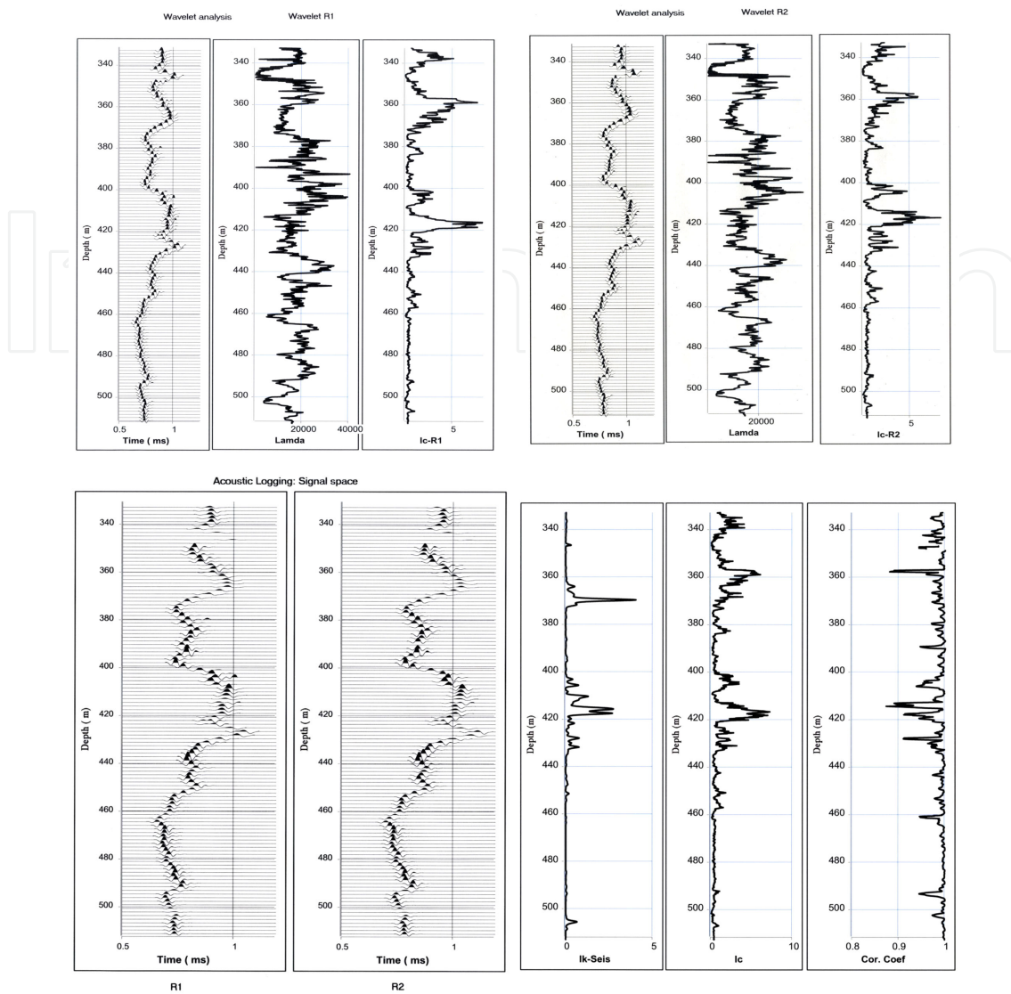
Figure 5. Analysis of refracted waves in acoustic logging by SVD [4]. Top : SVD analysis (Wavelet, amplitude, shape index) on receivers R1 and R2. Bottom from left to right: signal space (R1, R2); predicted permeability (Ik-Seis), shape index and correlation coefficient logs.
