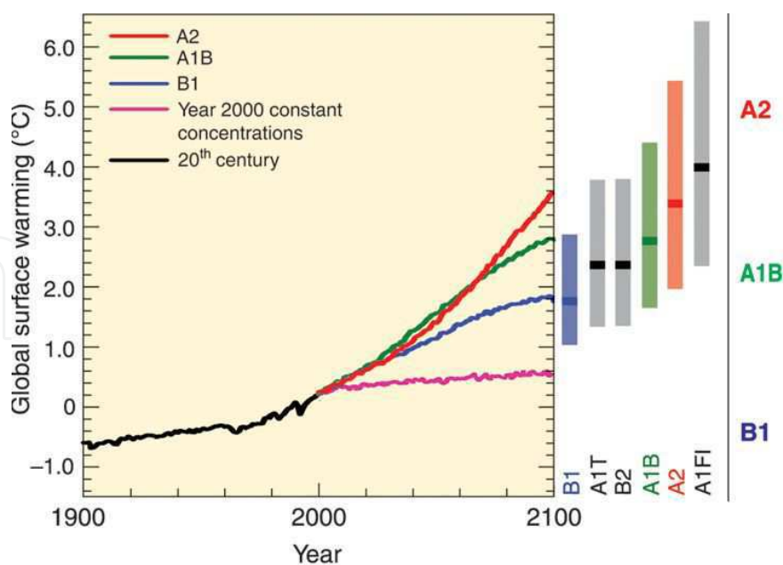
Figure 2. Scenarios of the global surface warming according to different emission rates of greenhouse gases; Source: IPCC Climate Change 2007: Synthesis Report Fig. 3-2.
