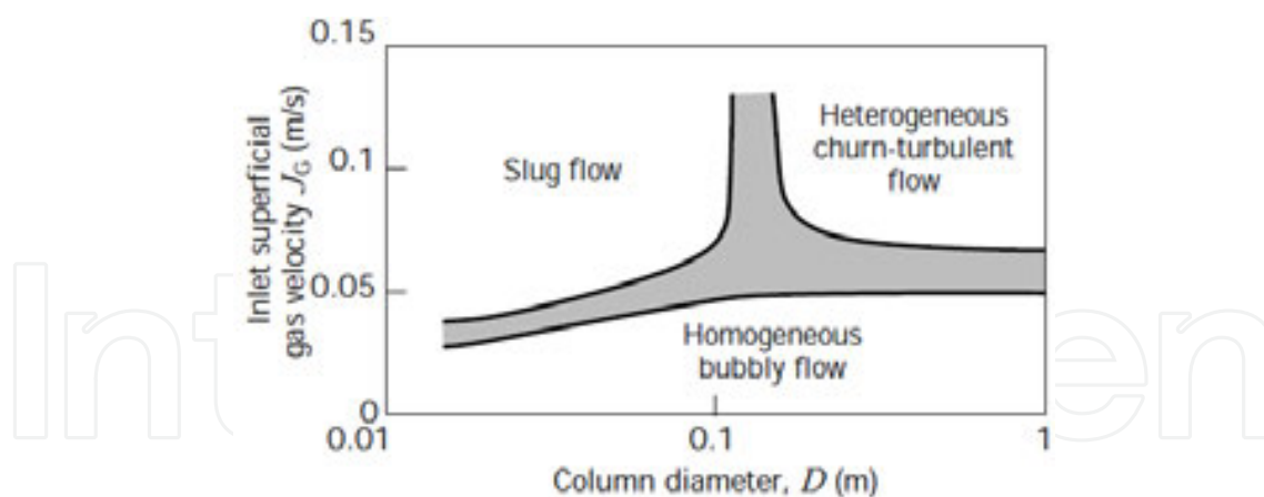
Figure 2. Map of flow configurations for gas–liquid concurrent flow in a vertical tube [12].
