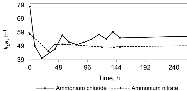
Figure 8. The evolution of k_L a through fermentation course employing two different nitrogen sources.
