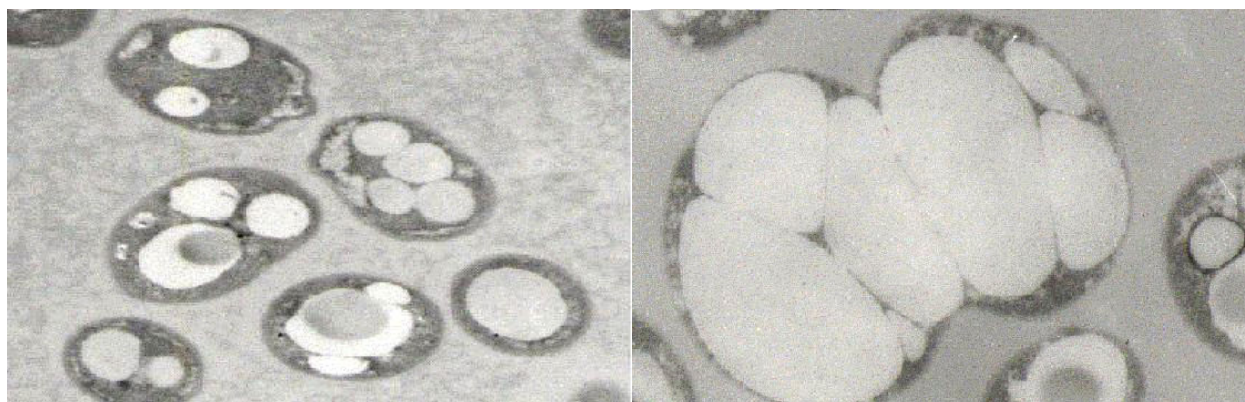
Figure 1. Exponential growth phase containing about 40 - 50% PHB (left) and final accumulation phase containing about 93% PHB (right).
