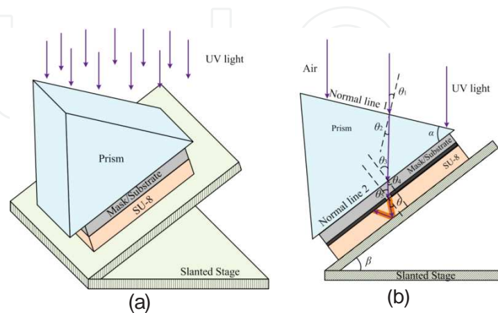
Figure 8. a) Schematic diagram of initiating cross-linking of the resin. (b) Schematic of cross-section view of the UV light path bending showing both incident and reflection exposures.
