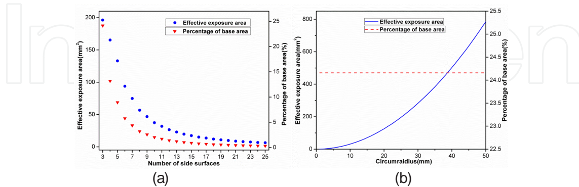
Figure 16. The effective exposure area and its percentage of base area (a) depend on the number of side surface and (b) depend on the circumradius of the base.
