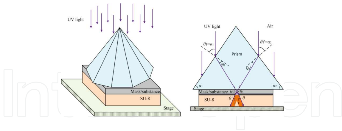
Figure 10. a) Schematic diagram of fabricating multi-directional structures using a polyhedron prism. (b) Schematic of a cross-sectional diagram showing the UV light paths.
