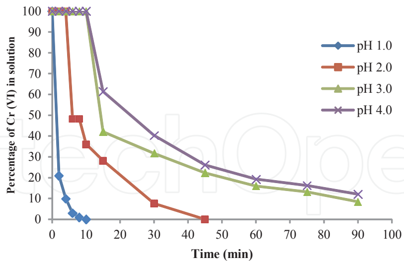
Figure 1. Effect of incubation time and pH on Chromium (VI) removal by L. chinensis Sonn shell. 100 mg/L Cr (VI). 28°C, 100 rpm. 1 g biomass.
