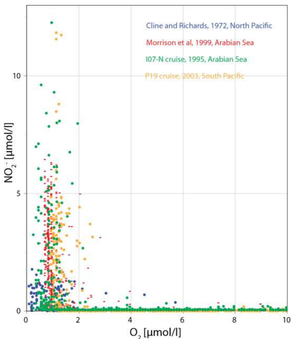
Figure 4. Dissolved oxygen versus nitrite for OMZs. Presented data are taken from publicly available cruises I07-N, P19 ( http://woce.nodc.noaa.gov/woce_v3/wocedata_2/bathymetry/default.htm ) and publications of Cline & Richards [182] and Morisson [183].
