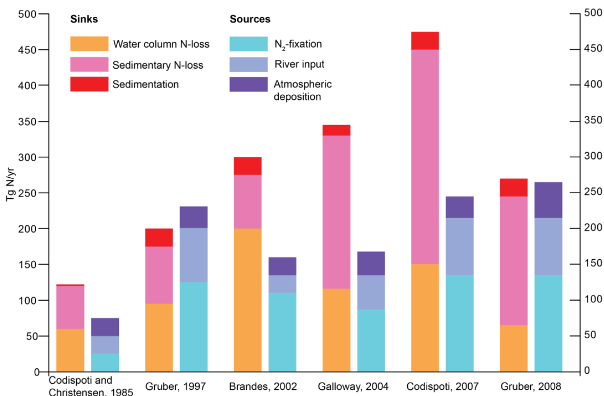
Figure 5. Nitrogen budget estimations in the literature.
