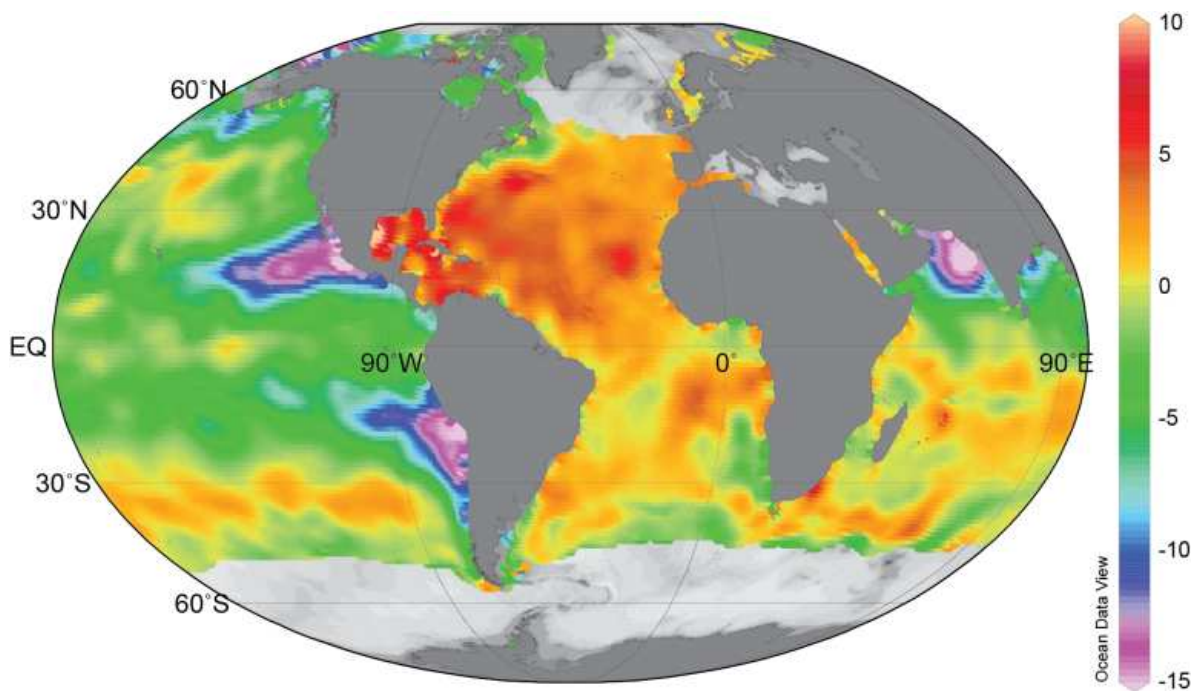
Figure 2. N^* = [NO_4^{3-}] - 16*[PO_4^{3-}] + 2.9 on the 26.5 sigma theta surface (World Ocean Atlas 2005). Note the large negative N^* values in the Tropical Pacific and Arabian Sea and positive N^* values in the Tropical Atlantic Ocean.
