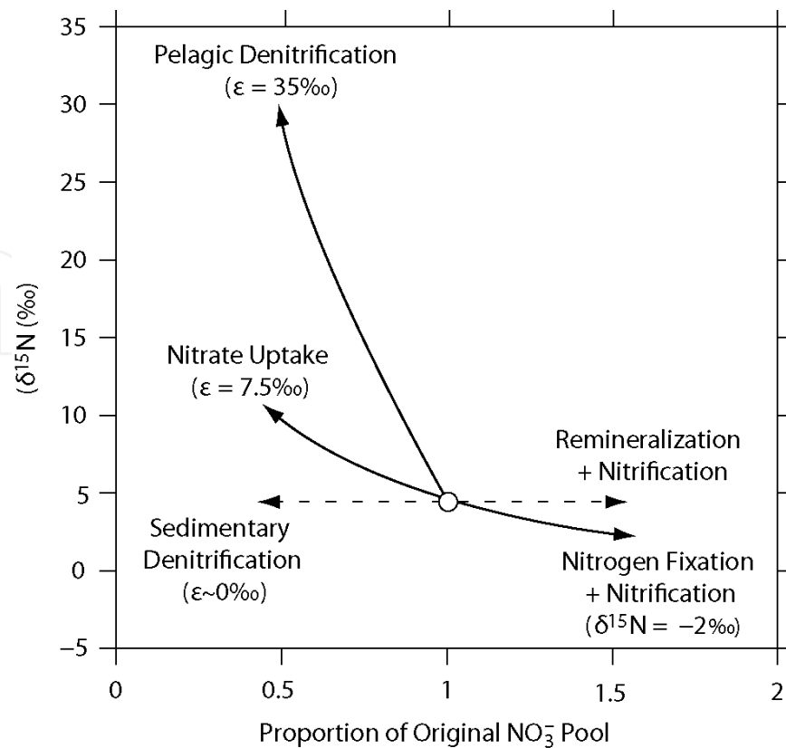
Figure 1. The impact of different processes on the \delta^{15}\text{N} of oceanic \text{NO}_3^- [56]. Axes show deviation of \delta^{15}\text{N} signal from oceanic average and loss/input of nitrogen due to different processes.
