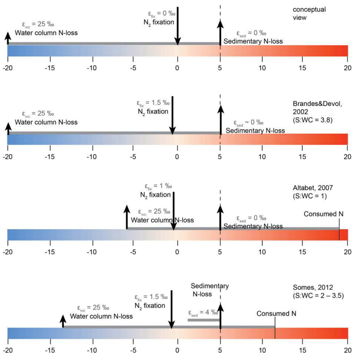
Figure 7. Nitrogen isotope range and processes influencing on the ^{15}\text{N} budget. Dashed line at 5‰ represent an oceanic average value [197, 202, 203].
