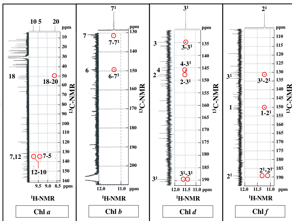
Figure 15. ^1\text{H} - ^{13}\text{C} -HMBC spectra of Chls a , b , d and f measured in acetone- d_6 at 273 K.
