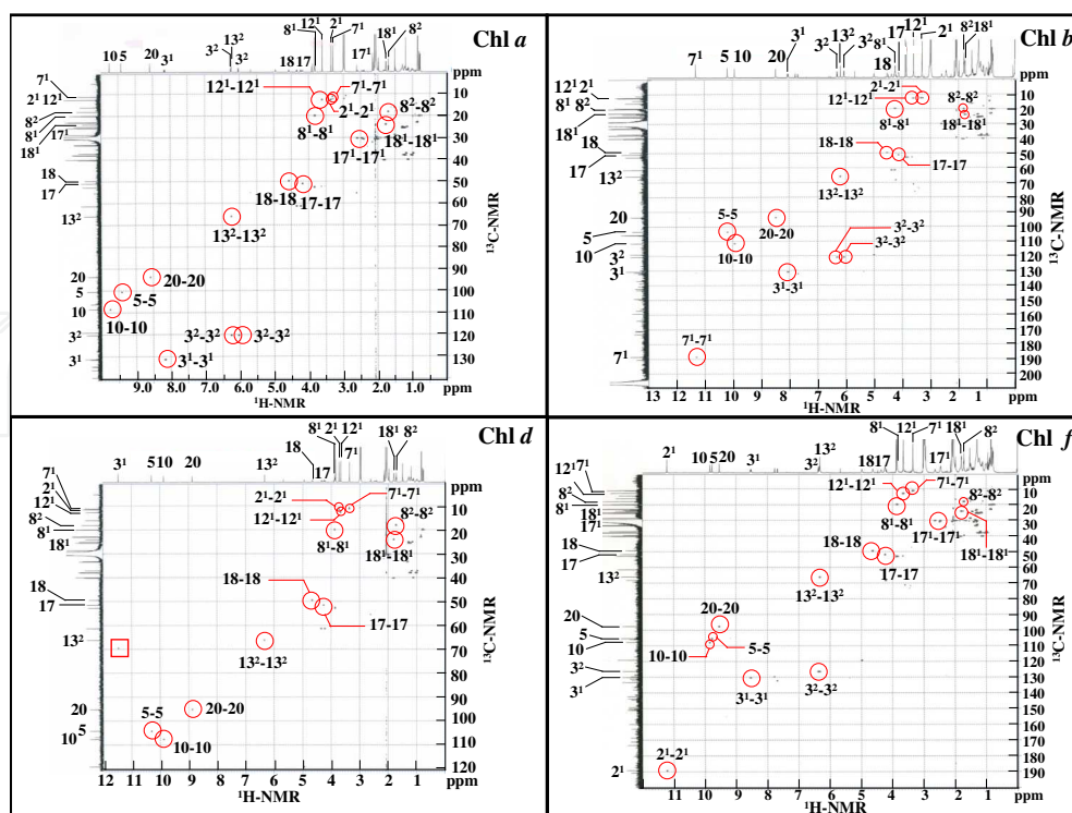
Figure 14. ^1\text{H} - ^{13}\text{C} -HSQC spectra of Chls a , b , d and f measured in acetone- d_6 at 273 K. \square in Chl d : \delta\text{C}189.59 (folded from outside the spectral window)
