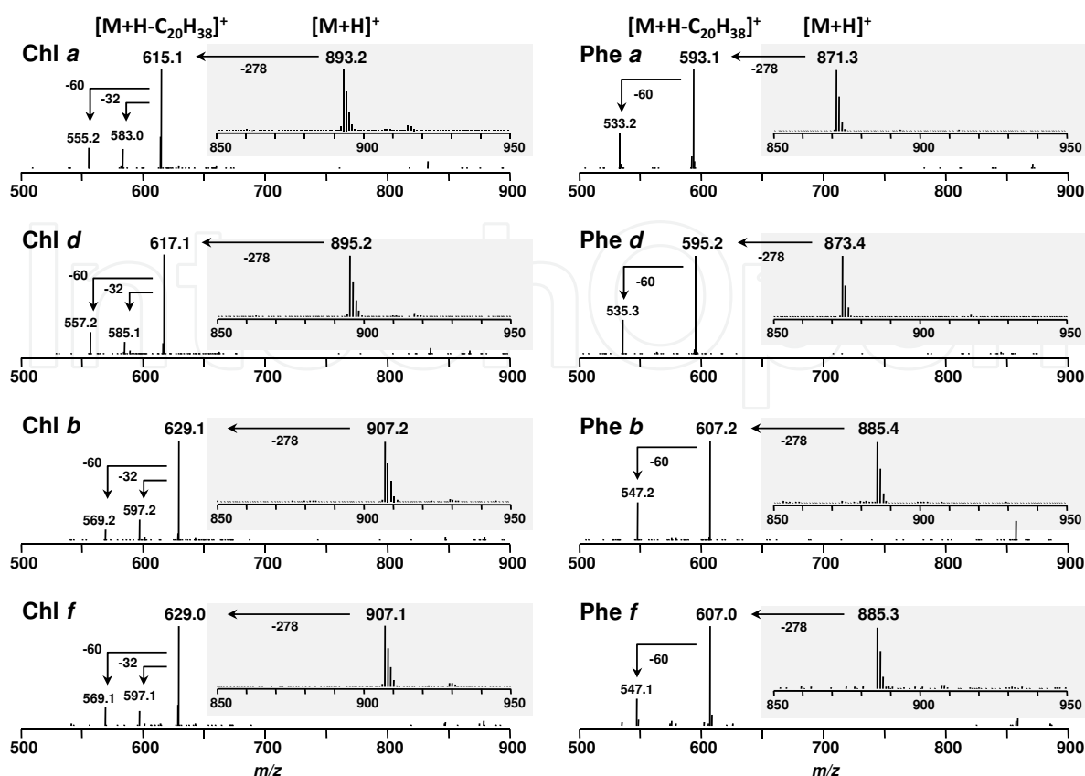
Figure 10. MS/MS spectra of Chls a , b , d , f (left column) and Phe s a , b , d and f (right column). Each mass spectrum of the chlorophyll fraction is shown in the shaded square. MS/MS spectra of the protonated molecules ( [M+H]^+ ) of Chls a , b , d and f give product ions of [M+H-278]^+ , [M+H-278-32]^+ and [M+H-278-60]^+ . Pheophytins a , b , d and f give product ions of [M+H-278]^+ and [M+H-278-60]^+ .
