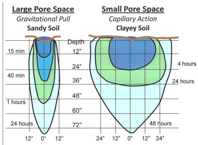
Figure 4. Comparative movement of water in sandy and clayey soils. In sandy soils, water readily moves downward due to the gravitational pull. In clay soils, water slowly moves in all direction by capillary action [8].
