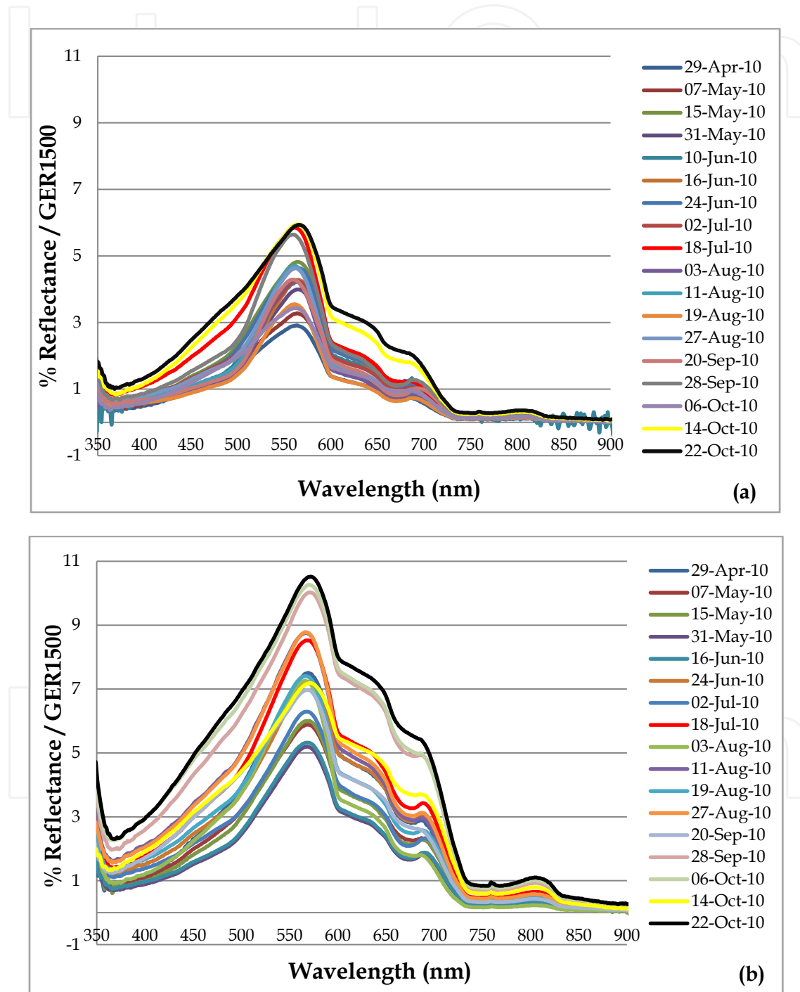
Figure 10. Typical Spectral signatures of (a) Outlet Area & (b) Inlet Area of Asprokremmos Dam acquired using a handheld field spectroradiometer GER1500.
