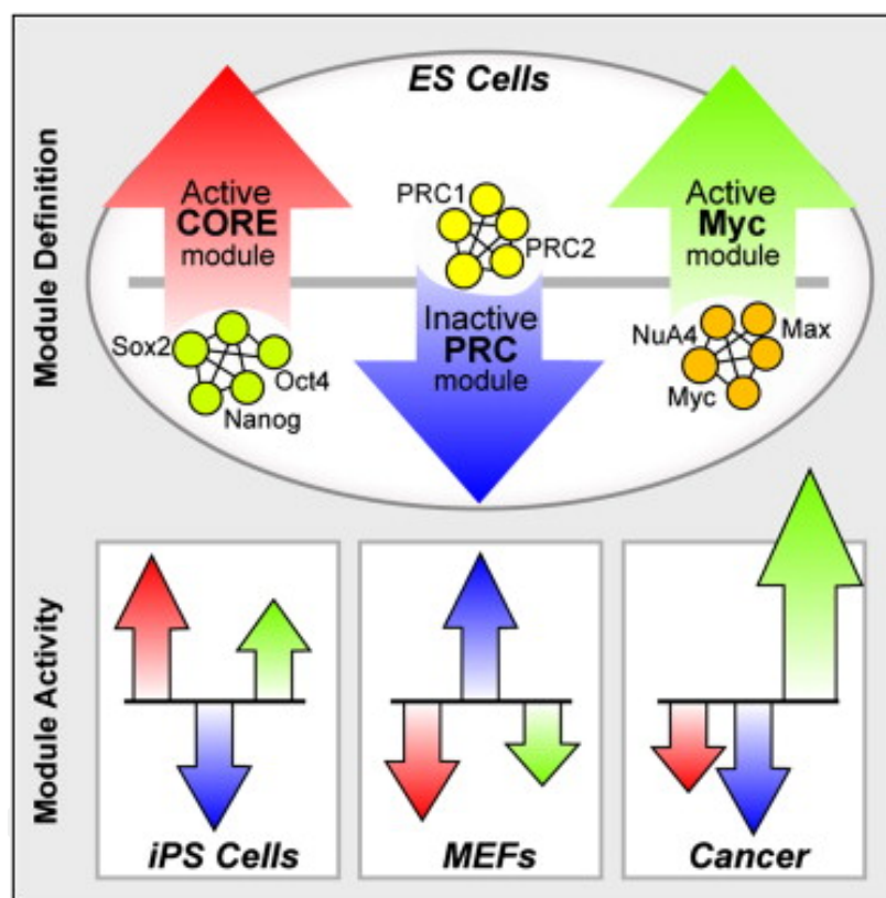
Figure 2. The three sets of genes that are activated or repressed by distinct sets of transcriptional regulators. Induce pluripotent stem (iPS) cells show similar gene expression profile as embryonic stem (ES) cells. Mouse embryonic fibroblast (MEF) represents a set of differentiated cells and shows a profile that is opposite to that of ES cells. Analysis of the profile in cancer highlights a pluripotency machinery in which the core module has been suppressed and the Myc module overactivated. Figure is a reprint of the graphical abstract provided by Kim et al [60] (Reprinted with permission from Cell Press)
