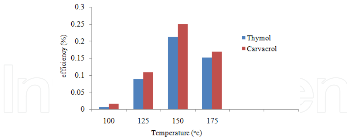
Figure 3. Effect of temperature on the main essential oil components SWE of Z. multiflora . Operating conditions: sample weight=4.0 g; flow rate=2 mL/min; particle size=0.50 mm; pressure=20 bar; and extraction time=60 min.
