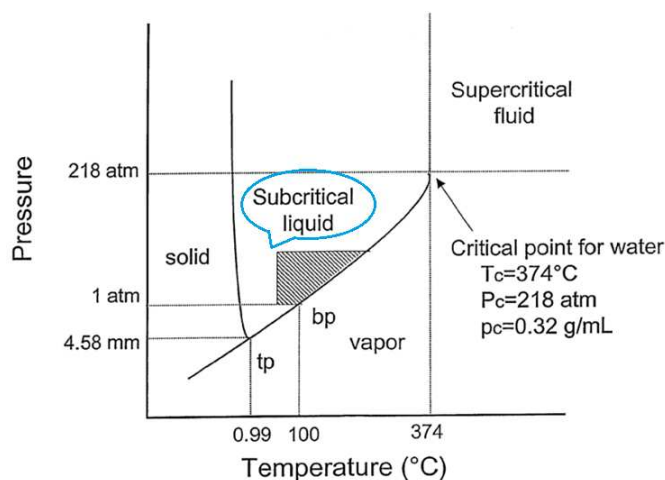
Figure 1. Phase diagram of water as a function of temperature and pressure (Cross-hatched area indicates the preferred region (SWE)) [4].
