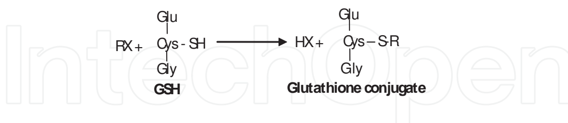
Figure 6. Representation of the conjugation reaction catalyzed by glutathione S-transferase (GST).
