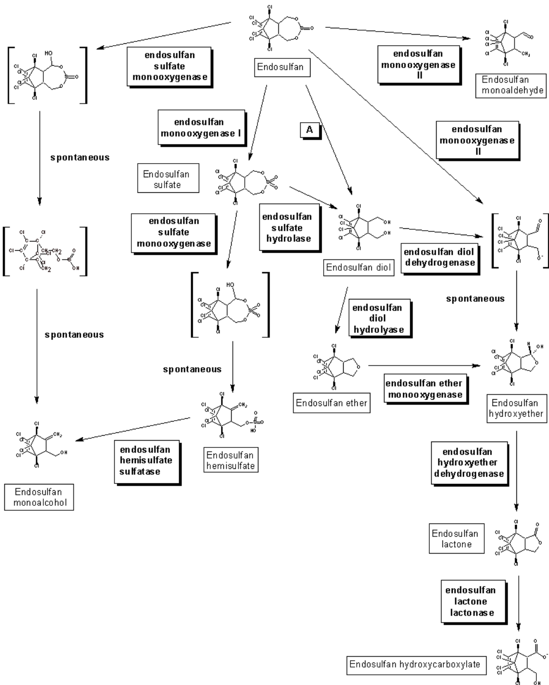
Figure 5. Degradation pathway of endosulfan (University of Minnesota. Biocatalysis/Biodegradation Database, http://www.umbbd.ethz.ch/end/end_map.html ).
