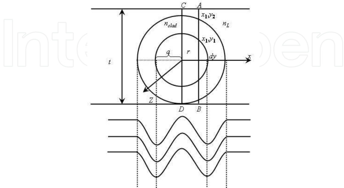
Figure 2. Cross section in a silvered liquid wedge interferometer with graded-index optical fiber of variable index core n(r) . A schematic representation of the resulting fringes is shown.
