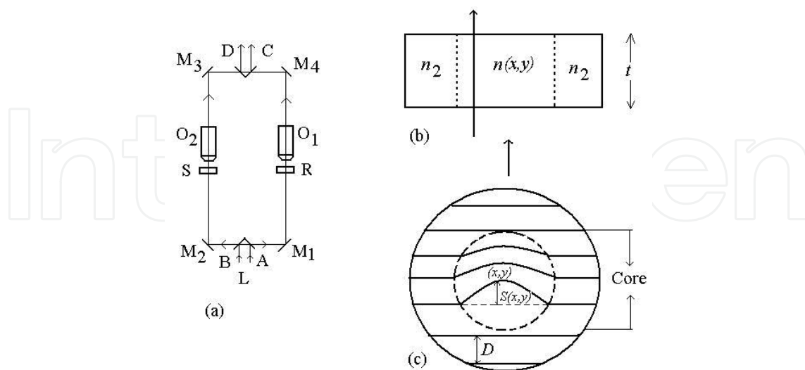
Figure 1. (a) A two-beam single-pass interference microscope. L is the incident light, M_1 , M_2 , M_3 , and M_4 are mirrors. S is the slab, R is the reference slab, O_1 and O_2 are microscope objectives. A, B, C, and D are semi-transparent mirrors. (b) A slab of thickness t for a graded-index core with a cladding of refractive index n_2 . (c) Interferogram in which the fringe shift Z(x, y) in the core region is a function of point position x, y is shown.
