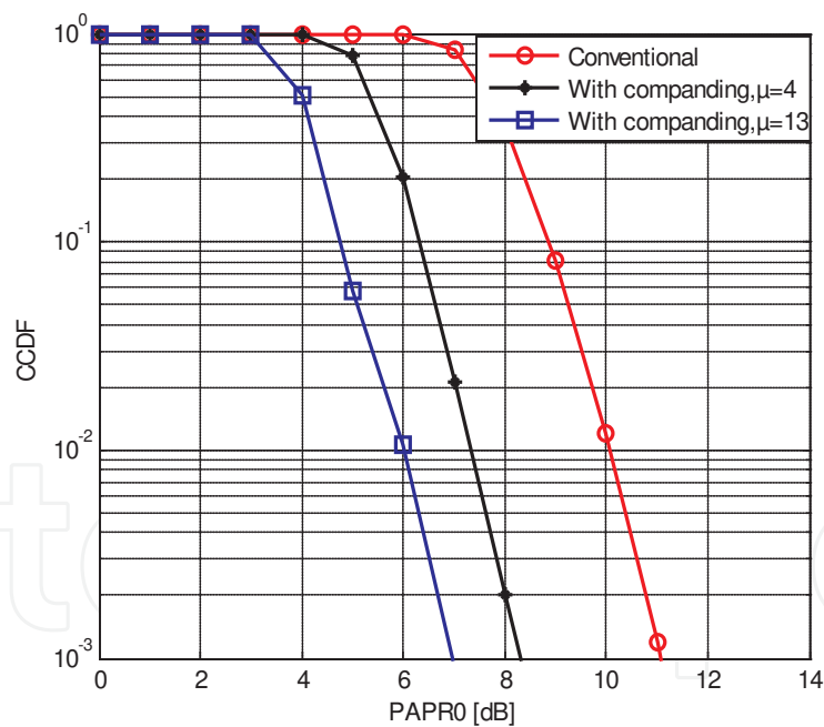
Figure 16. CCDF of PAPR with the proposed system (64QAM).
