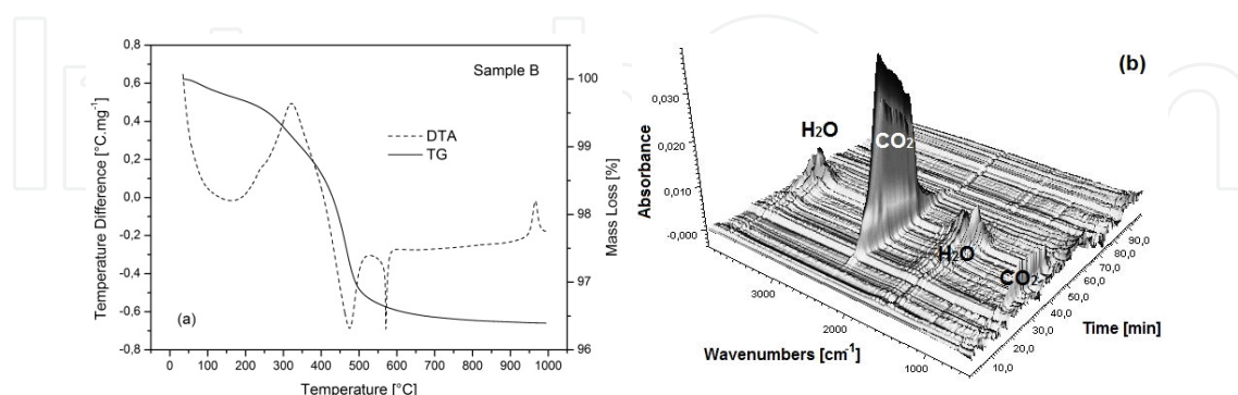
Figure 15. Thermal analysis of the sample B: TG-DTA (a) and EGA (b).
