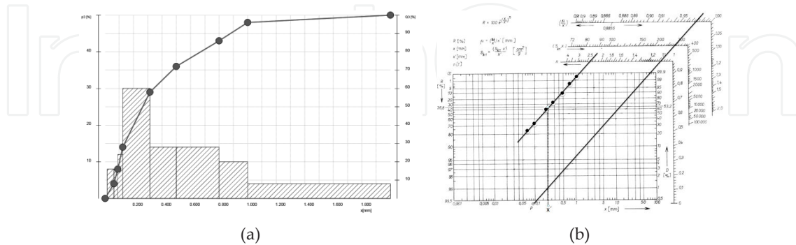
Figure 6. The sieve analysis of the Sample C (a) and RRSB diagram (b)
