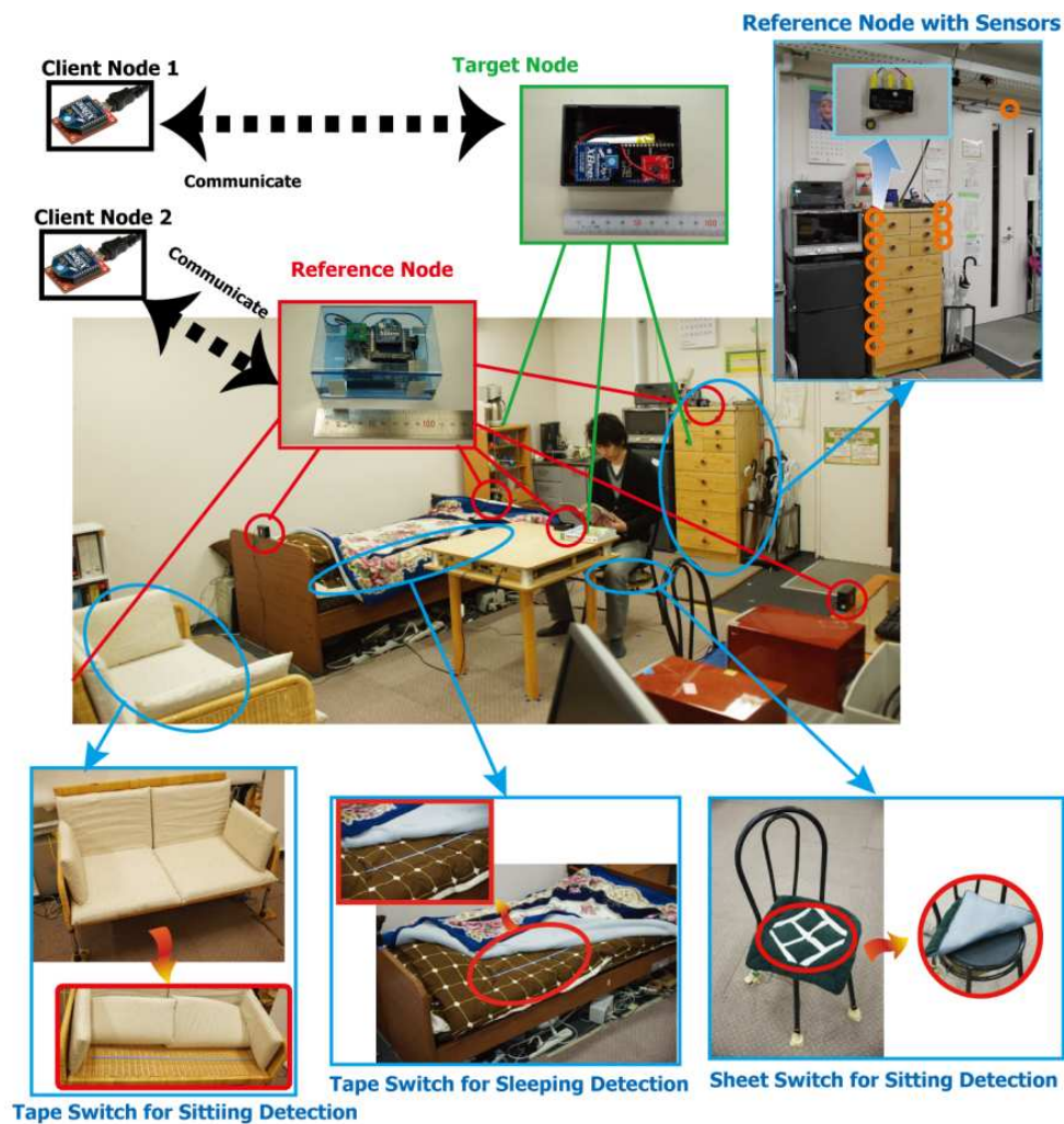
Figure 1. Developed devices and deployment examples.
