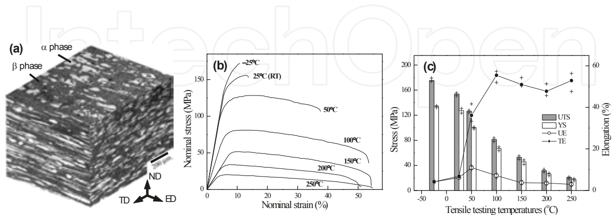
Figure 13. (a) Optical micrograph of as-extruded LAZ1021 base metal at the ND, ED and TD planes, (b) stress-strain curves, and (c) tensile testing results of the LAZ1021 alloy at various temperatures.
