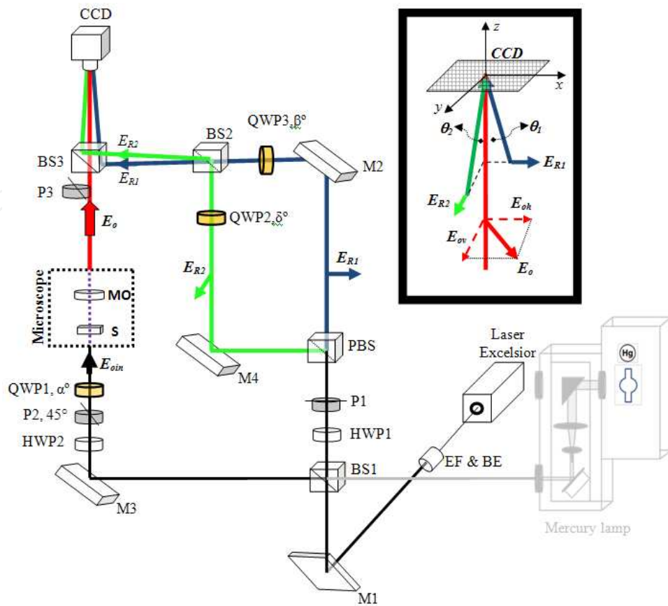
Figure 4. Schematic diagram of the Polarization Holographic Microscope for the study of linear dichroism and birefringence (symbology described in the text).
