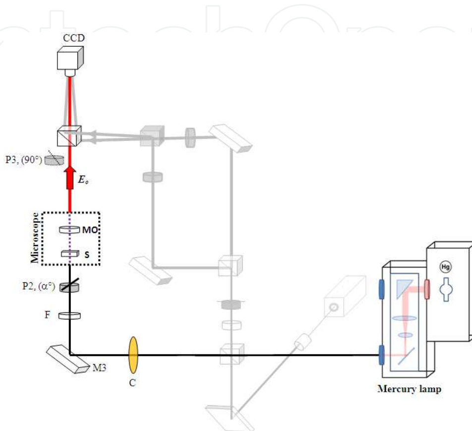
Figure 2. Differential Polarization Microscope. Light source is a mercury lamp, M3 is a mirror, C is the condenser system of the light beam, F is an interferential filter, P2 is a polarizer, S is the sample, MO is the objective lens and CCD is the digital capture device.
