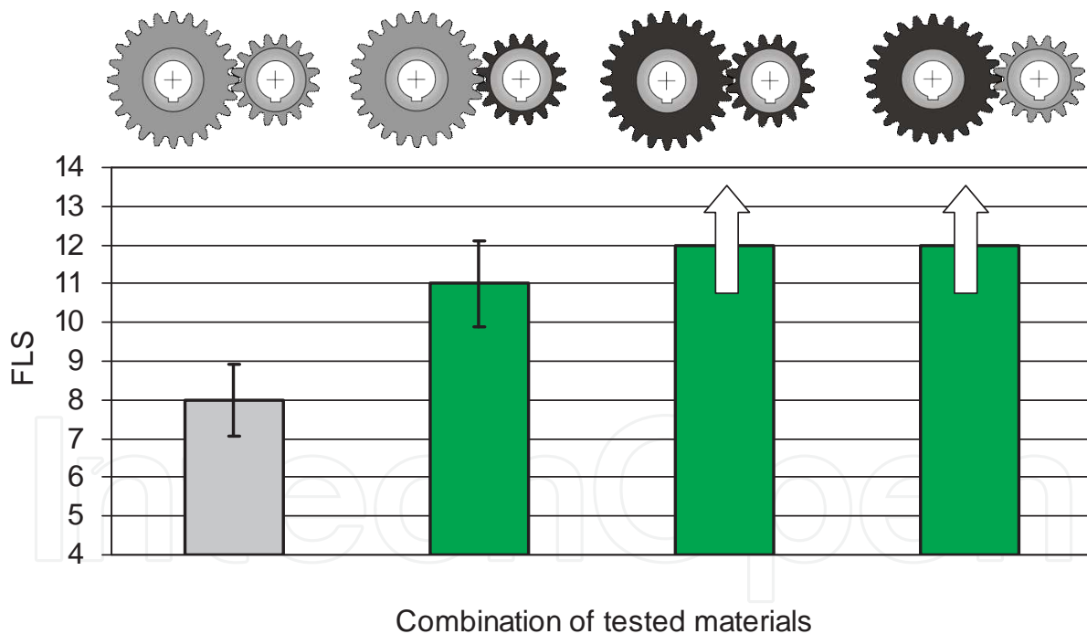
Figure 14. Failure load stages (FLS) obtained using the Gear Scuffing Shock Test for Coatings for the tested material combinations with the MoS 2 /Ti coating
