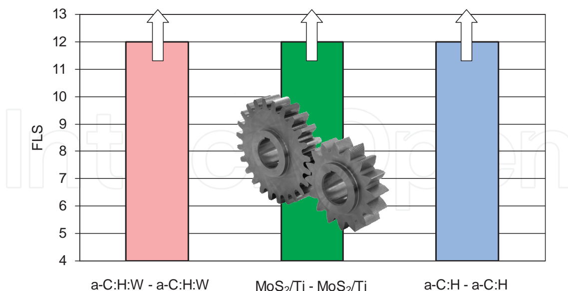
Figure 5. Failure load stages (FLS) obtained for the tested coatings (both gears coated) - FZG A/8.3/90 test method; data compiled from [23-25]
