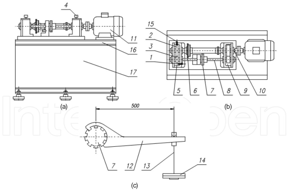
Figure 9. Kinematic schemes of the T-12U gear test rig: a) front view, b) top view, c) loading equipment; 1 - thermocouple, 2 - test wheel, 3 - test pinion, 4 - vent, 5 - test chamber, 6 - shafts torsion angle indicator, 7 - load clutch, 8 - front shaft, 9 - slave chamber, 10 - drive clutch, 11 - electric motor, 12 - loading lever, 13 - weight hanger, 14 - weights, 15 - heaters, 16 - frame, 17 - concrete base
