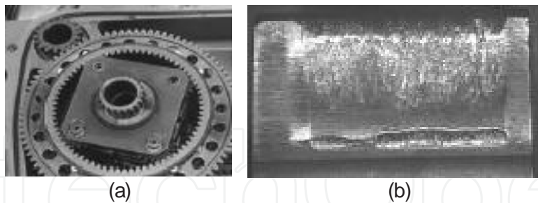
Figure 2. Photographs of the components of the rudder speed brake power drive unit of a space shuttle: a) pinion and ring gear of the power drive unit, b) damaged pinion tooth [4]
