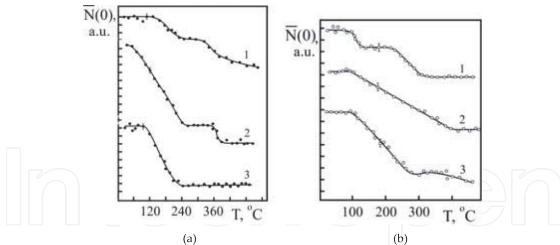
Figure 15. Kinetics of Ti (a) and Ti-7.6 at% Sn alloy (b) annealing under different types of exposure. 1 – deformed by \epsilon = 50\% ; 2 – irradiated by protons in a deformed state; and 3 – the same in an annealed state.
