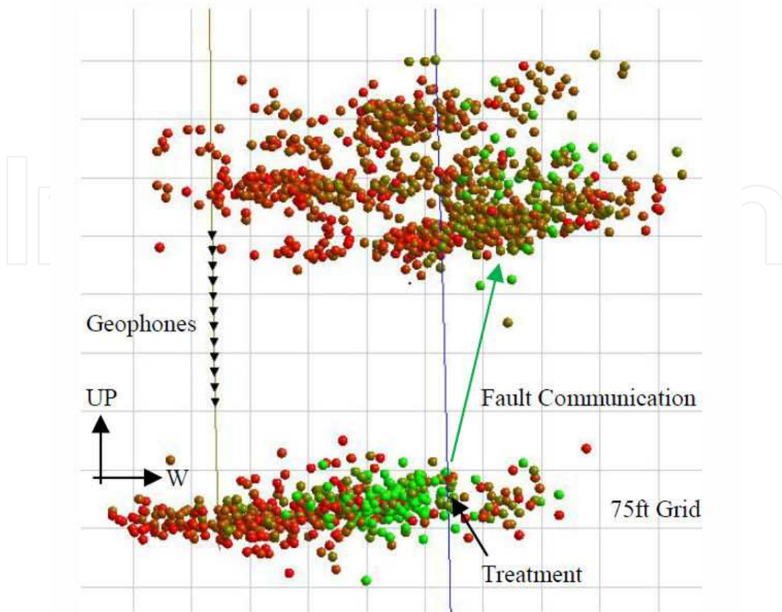
Figure 5. Hydraulic fracturing of a tight-gas sand. 1408 events are recorded over 5 hours. Events are colour shaded by time: green (earliest) to red (latest). Events occur in two formations with very few detected events in between. Yet the event history reveals that brittle failure occurs first in the right-most part of the bottom formation, and then suddenly jumps to the top formation indicating the presence of a possible aseismic fault. After Pettitt et al. (2009).
