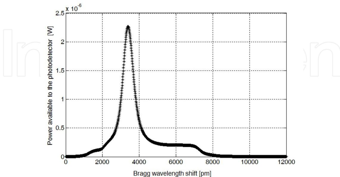
Figure 16. The convolution between F_{FP}(\lambda) * F_{FBG}(\lambda) .
