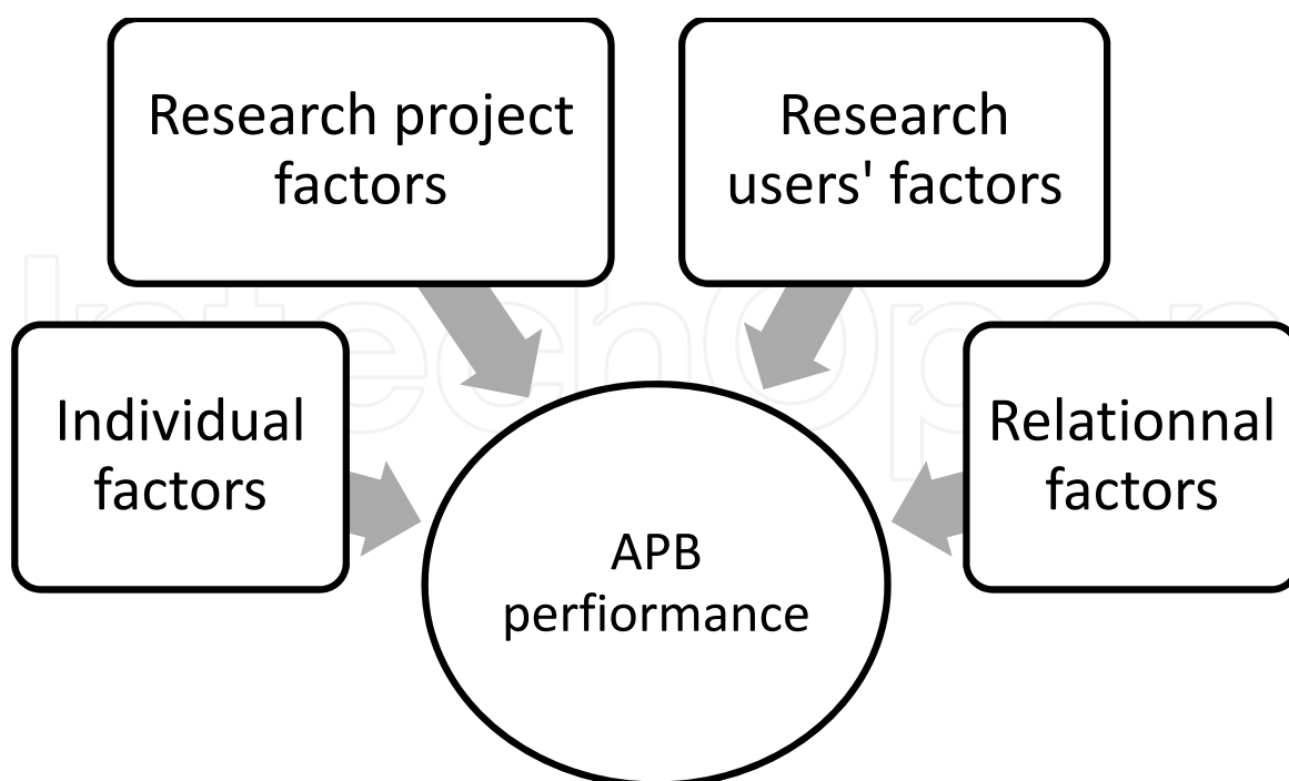
Figure 1. Operational framework
