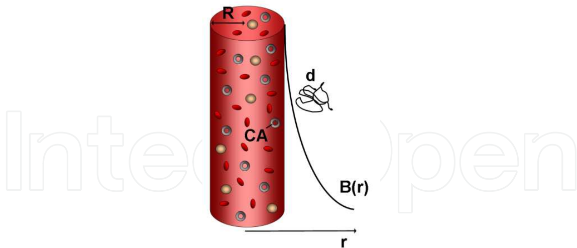
Figure 3. The \Delta R_2^* method for CBV measurement models the capillary as an infinitely long and homogeneous cylinder containing the CA. The magnetic field gradient around the cylinder is a function of the cylinder radius R , of the magnetization difference between the intra- and extravascular compartment, of the cylinder orientation in the main homogeneous magnetic field B_0 and of the distance from the cylinder r . The diffusion regime is said to be quasi static when the mean water proton diffusion length d is short with respect to R , in such a way that the water protons in the vicinity of the cylinder dephase at a faster rate than those situated further away.
