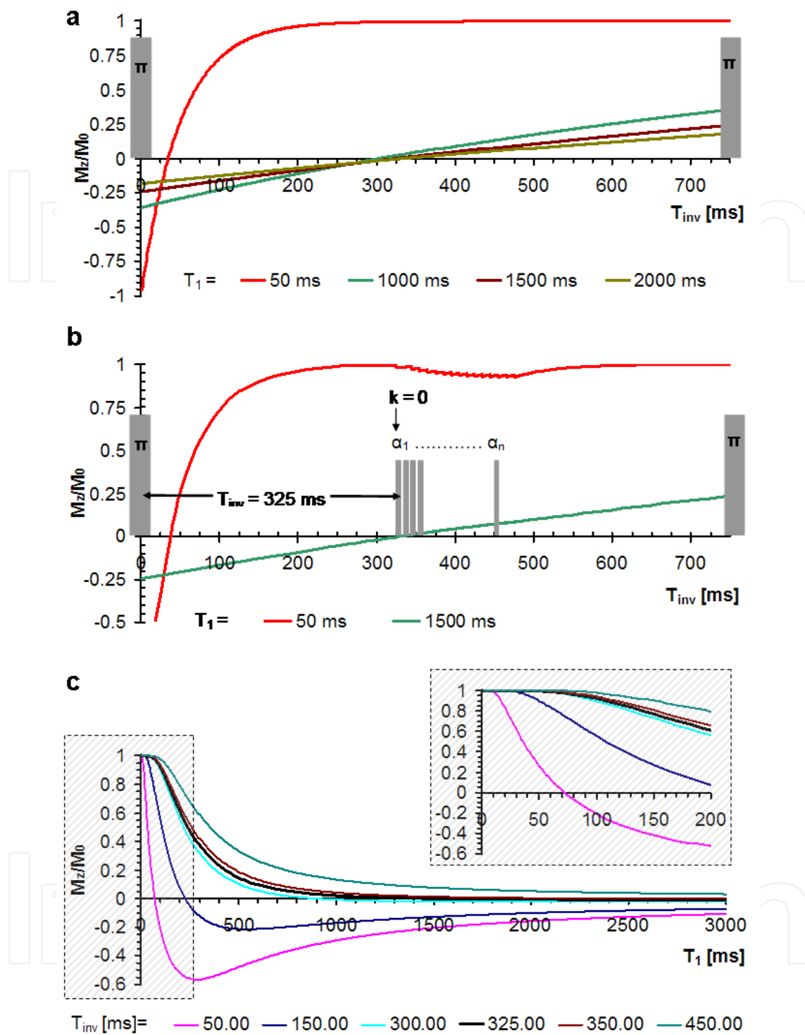
Figure 4. a: The longitudinal magnetization component M_z in an IR sequence with 750 ms repetition time is plotted after dynamic equilibrium has installed. M_z is suppressed and crosses the zero line at almost the same T_{inv} for tissues with long T_1 , while for the same T_{inv} M_z is at thermodynamic equilibrium for tissues with short T_1 such as blood in presence of the CA. \pi = nonselective inversion pulse. b: The FLASH module acquires the image (and in particular the k = 0 line) when M_z of tissues with long T_1 crosses the zero-line and blood magnetization is fully relaxed (due to the T_1 shortening effect of a vascular CA). Here a center-out acquisition scheme is illustrated. \alpha = low flip angle pulse. c: Equation 4 is plotted as a function of T_1 for several T_{inv} and TR = 750 ms. For T_{inv} = 325 ms M_z is suppressed for all T_1 \geq 1 s while it relaxes to thermodynamic equilibrium for T_1 \leq 65 ms as shown in the zoom.
