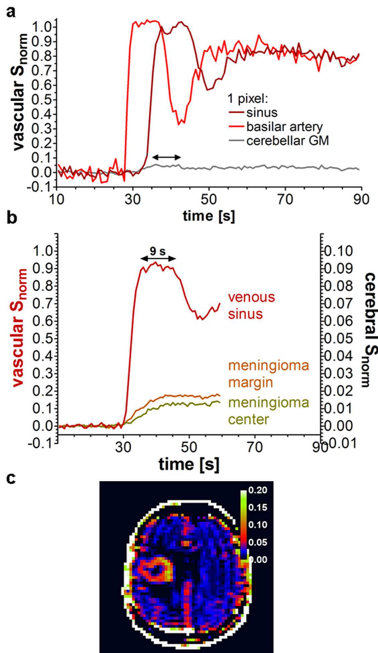
Figure 11. a: After an intravenous Gd-DOTA injection of 0.13 mmol/kg in patients, S_{\text{norm}} = 1 is attained during the first pass in large vascular structures without partial volume effect. The S_{\text{norm}} amplitude in brain tissue during the first pass (arrow) therefore corresponds to the BVf. S_{\text{norm}} = 0.04 in the cerebellar gray matter (GM) voxel. b: While the vascular signal is in a RSS for about 9 s in this patient, a typical CA leakage profile is observed in the meningioma tissue. c: S_{\text{norm}} map of a patient with glioblastoma. No leakage correction was applied and the BVf of 8 to 10% in the tumor border might be overestimated if significant CA leakage occurred during the first pass.
