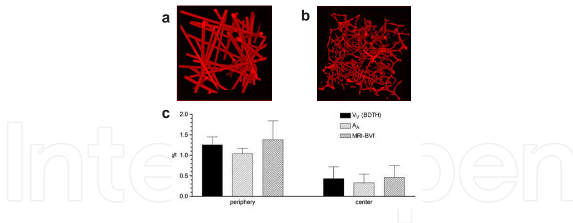
Figure 12. Validation of the C6 tumor BVf measured with Gd-ACX and the RSST 1 technique. a and b: Numerical models used to evaluate the stereological approach: cylinder model (a) and cortical mouse vasculature (b). The stereological analysis of vascular morphometry confirms the tumor BVf measured by MRI (c).
