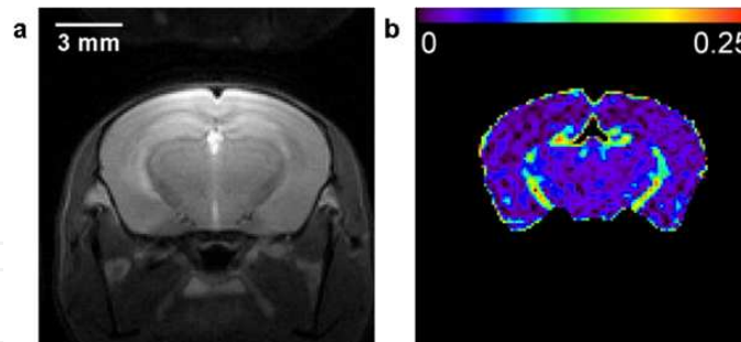
Figure 6. a: Coronal MRI image of a mouse brain showing structural details. b: Corresponding S_{norm} map showing an average cerebral BVf of 0.02 \pm 0.004 and demonstrating CA accumulation in the cerebrospinal fluid leading to overestimation of the CBV in periventricular structures.
