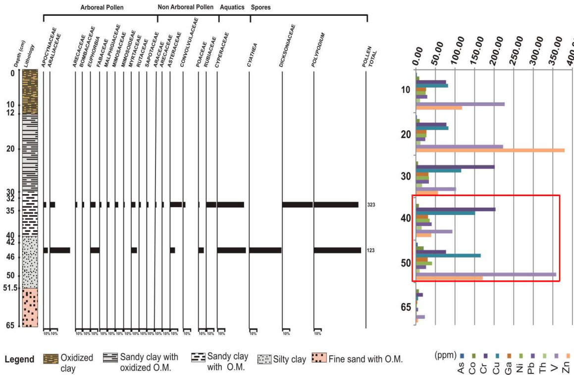
Figure 2. Descriptive profile of the T-UNICAMP core featuring a pollen diagram and the distribution of trace elements (T.E.) in depth.
