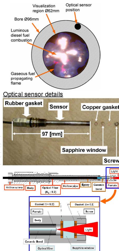
Figure 7. Optical sensor location and design
