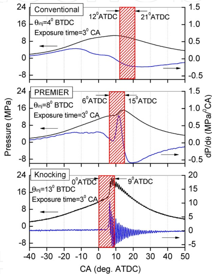
Figure 8. In-cylinder pressure and the rate of pressure rise. P_{inj}=40 MPa, P_{in}=200 kPa, D_{hole}=0.1 mm, N_{hole}=3 , m_{air}=2 mg/cycle, \phi_t=0.6
