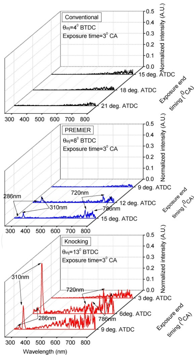
Figure 9. Detailed spectra in the end-gas region. P_{inj}=40 MPa, P_{in}=200 kPa, D_{hole}=0.1 mm, N_{hole}=3 , m_{air}=2 mg/cycle, \phi_t=0.6
