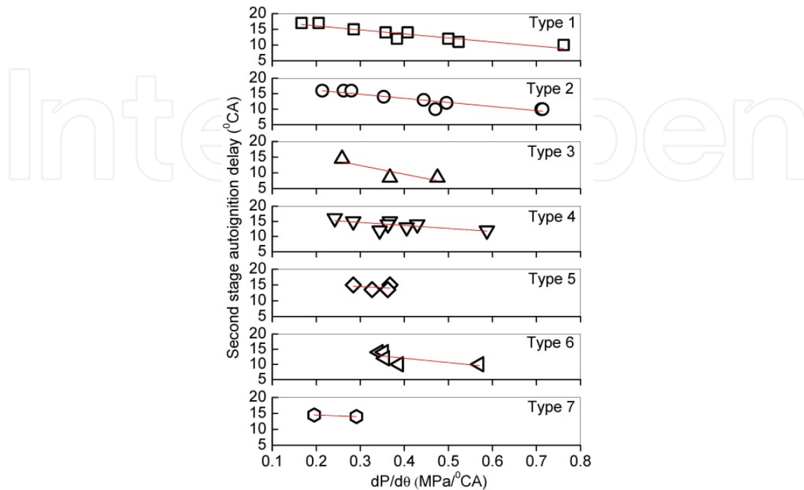
Figure 14. Second stage autoignition delay. P_{inj}=80 MPa, P_{in}=200 kPa, m_{df}=3 mg/cycle
