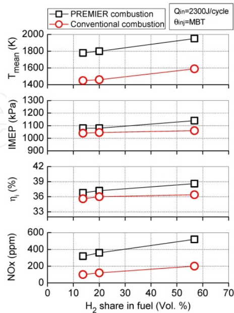
Figure 17. Effect of H_2 content on engine performance characteristics at \theta_{inj}=\text{MBT}
