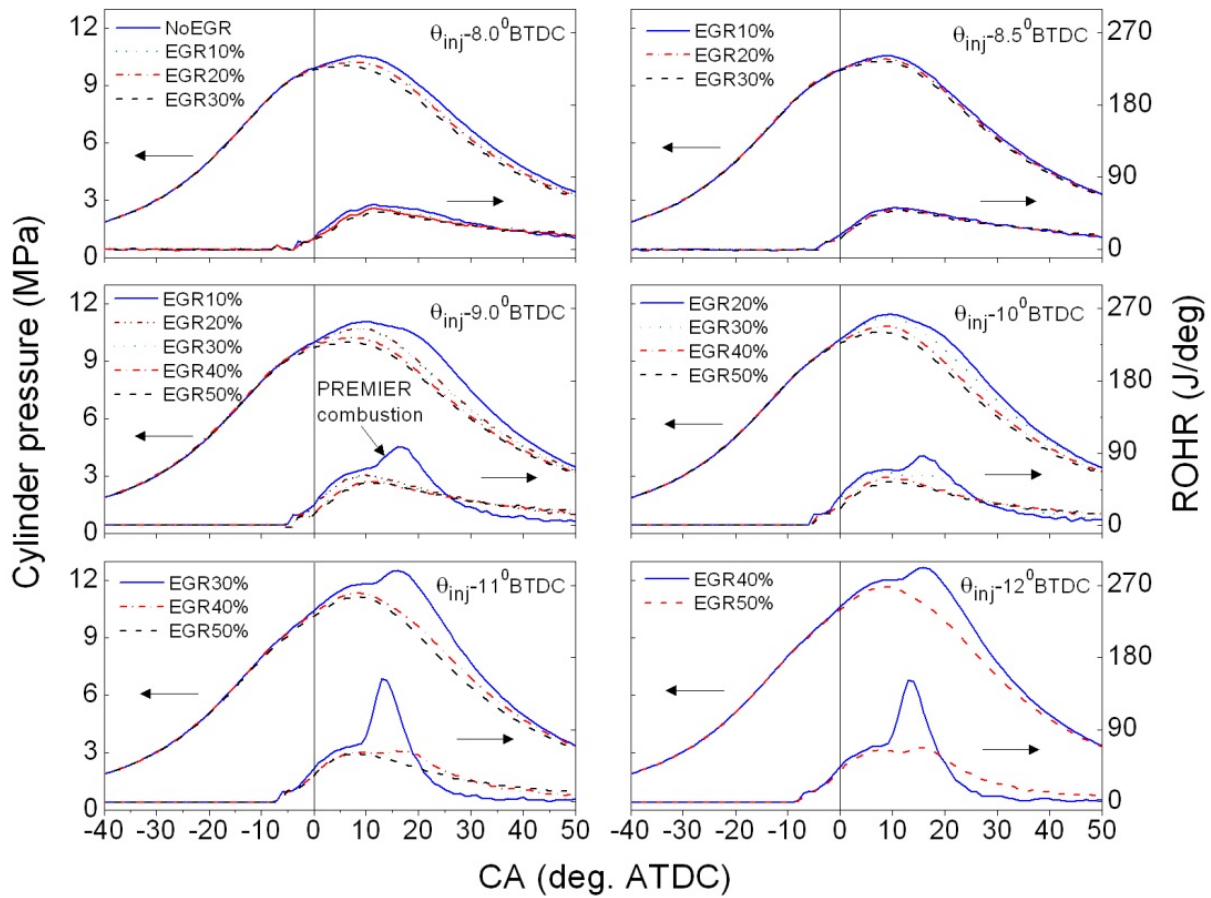
Figure 12. Effect of EGR on cylinder pressure and the rate of heat release. P_{inj}=40 MPa, P_{in}=200 kPa, D_{hole}=0.1 mm, N_{hole}=3 , m_d=2 mg/cycle
