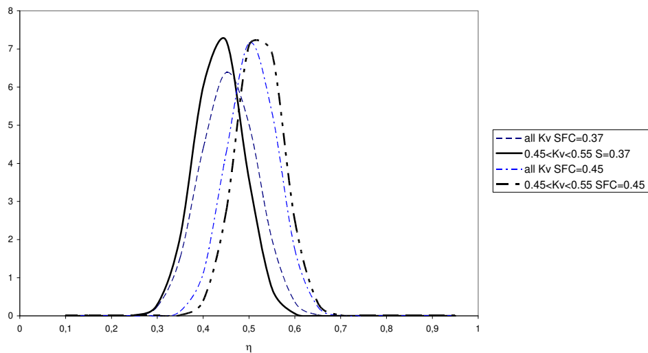
Kernels of \eta with assumptions on SFC and Kv (Sejnane)
