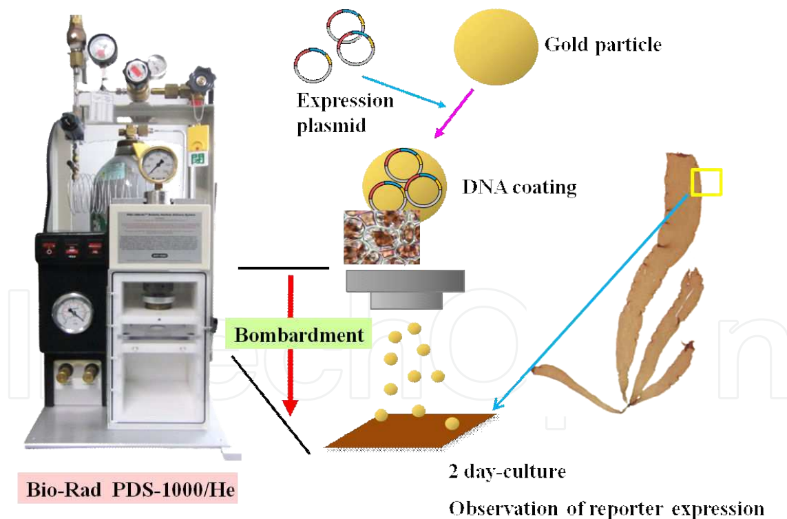
Figure 2. The established procedure of transient transformation in P. yezoensis . A circular expression plasmid is bombarded into P. yezoensis gametophytic cells using the Bio-Rad PDS-1000/He after coating of gold particles with the plasmid. Expression of the reporter gene is observed after cultivation of the bombarded gametophyte under dark for two days; for PyGUS reporter gene, histochemical staining with X-gluc solution and fluorometric analysis of enzymatic activity are performed; for fluorescent reporter genes, bombarded samples are examined with fluorescent microscopy.
