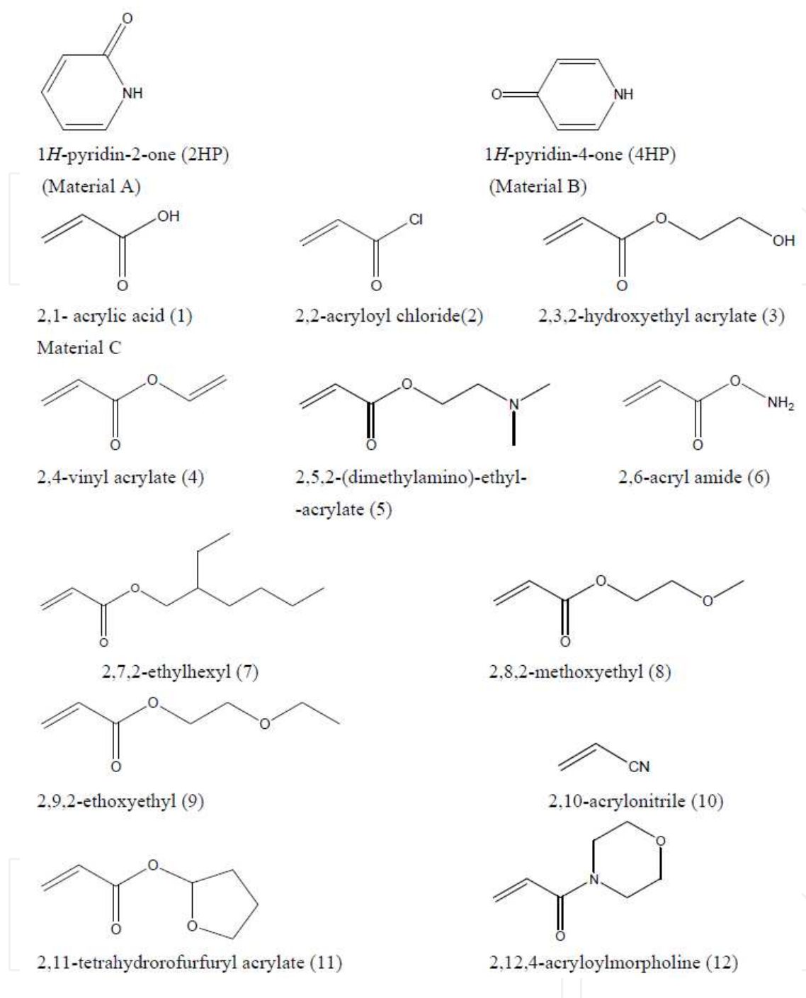
Figure 3. Chemical structures of materials for propionate synthesis
