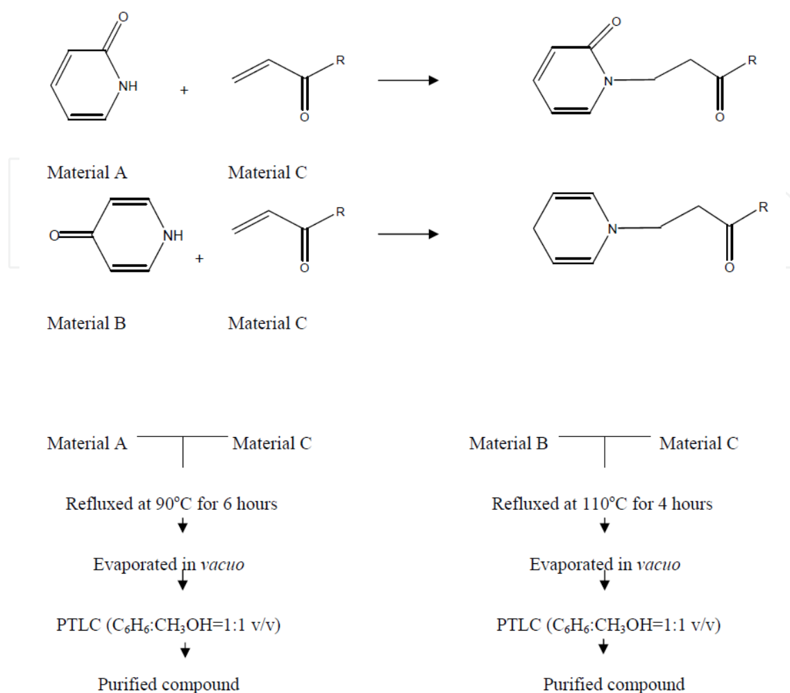
Figure 4. Synthesis route of propionates
