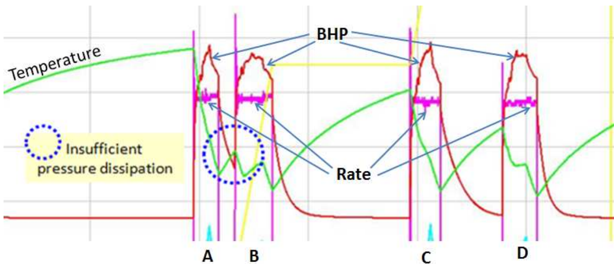
Figure 5. Pressure responses from four injections where the red line is bottom-hole pressure (BHP), the pink line is injection rate, and the green line is temperature. Pressure dissipation for injection A is insufficient. Pressure dissipations for injections B, C, and D are sufficient. The temperature drop validates the entry of injection fluid at the perforation.
