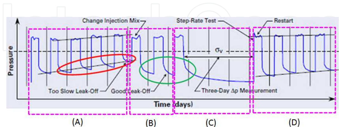
Figure 1. Pressure responses over long period of cuttings injection. (A): gradual pressure build up due to insufficient fracture closing; (B): good fracture closing; (C): excellent fracture closing with sufficient time; and (D): gradual pressure build up due to insufficient fracture closing.
