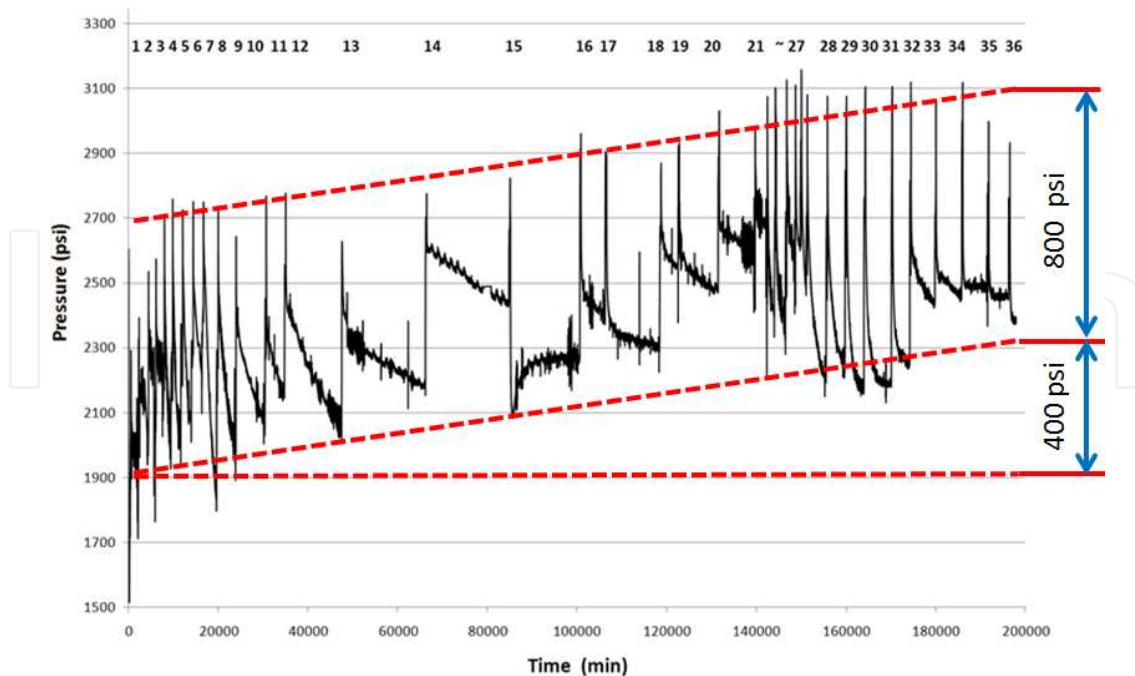
Figure 3. Observed WHP over 36 injection batches with an average pressure increase of 400 psi and differences between peak WHP and terminal WHP of 800 psi. The rate of pressure increase is 50%.
