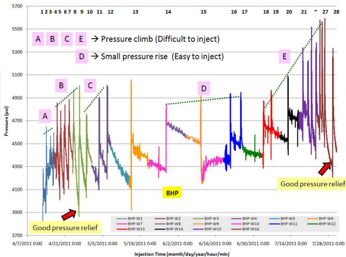
Figure 2. Observed bottom-hole pressures during 28 injection batches. Durations A, B, C and E show the rising peak pressures that are the indication of difficulties in cuttings injection. Duration D shows a slight rise of peak pressure that is the indication of easier cuttings injection.
