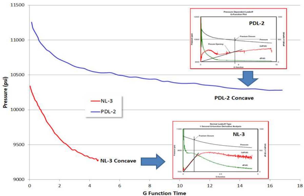
Figure 11. Comparison of two cases of (NL-3 and PDL-2): a) initial linear line and late linear line with a different slope for the P - G relationship with normal leakoff; and b) concave curves for the P - G relationship with pressure-dependent leakoff.
