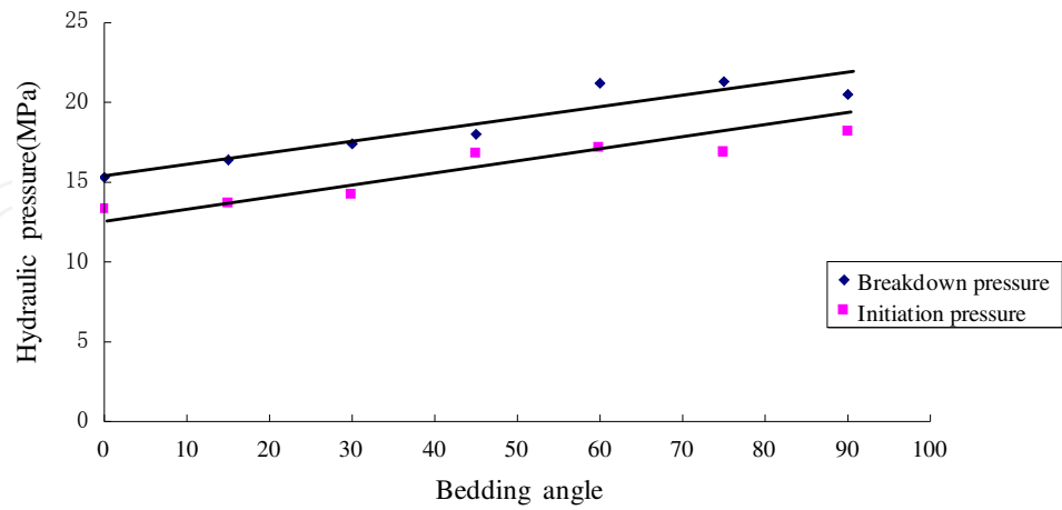
Figure 20. Changes of initiation and breakdown pressure of different bedding angle specimens
