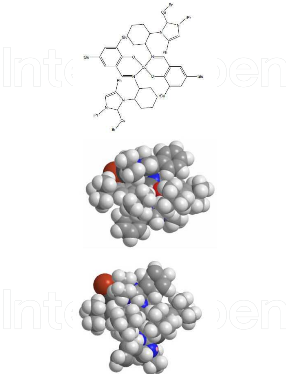
Figure 12. CCDC YUBLAJ [23]. The compound has a formula C_{66}H_{88}Br_2Cu_3N_6O_2 . Novel feature mentioned is that it appears that problematic deprotonation of the phenol to give a chelating or bridging ligand is the primary reason for the observed instability based on the stability of related copper NHC–aryl oxide compounds (including mixed valence Cu(I)/Cu(II) centers Cu(I) sites in ligands) Apparently conformational change was from a step and slightly twist form to an umbrella and twist (about 90 degree) form.
