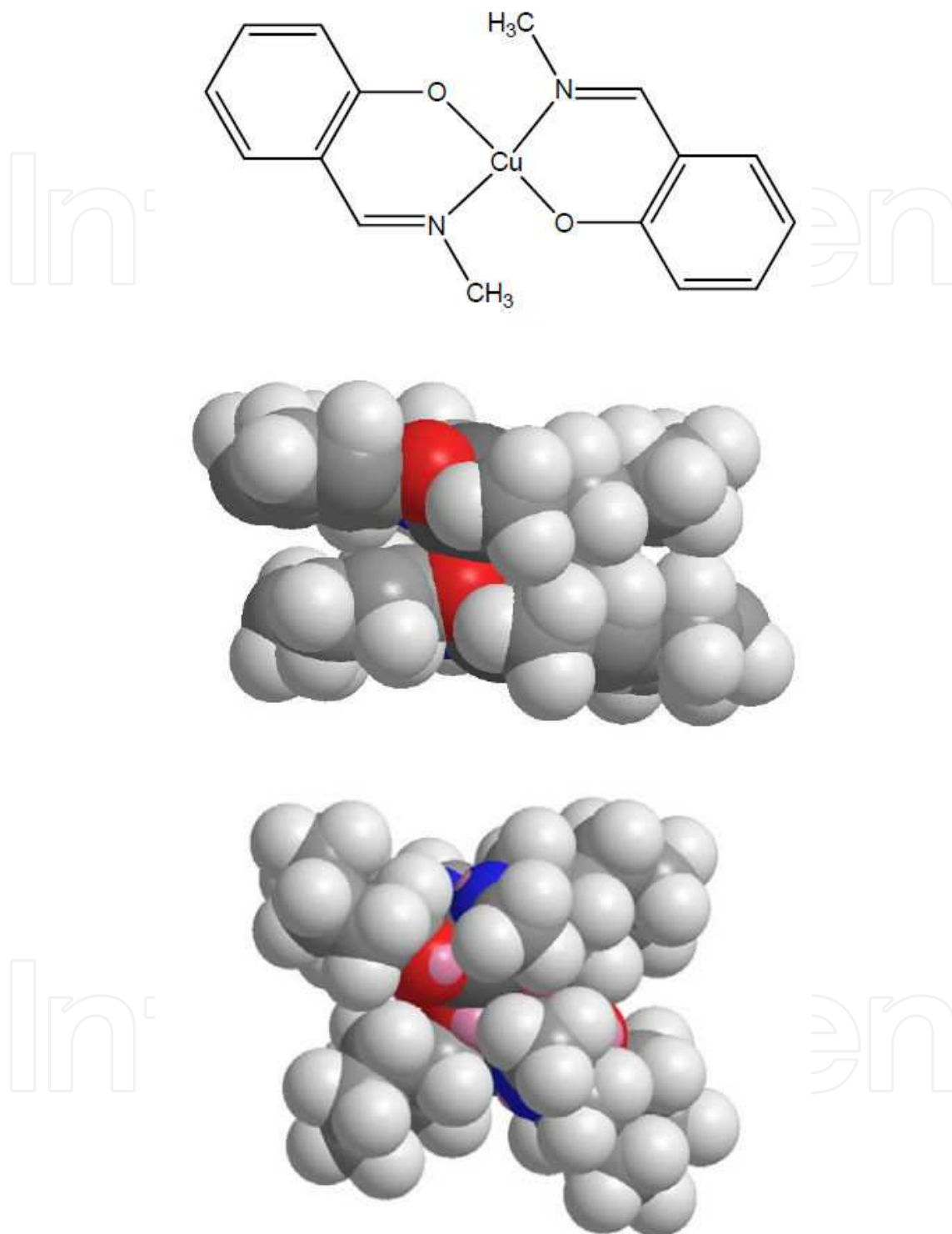
Figure 8. CCDC MSACOP12 [22]. The compound has a formula C_{16}H_{16}CuN_2O_2 . Novel feature mentioned is that a dimeric molecule in which monomeric halves is joined by two Cu-O bonds to complete a square-pyramidal configuration about each copper atom. Distortions in the molecule are evidently due to the close approach of non-bonding regions. It is now seen that this compound displays three different coordination arrangements in its three polymorphic forms. Apparently conformational change was from a step form to an umbrella and twist (about 45 degree) form.
