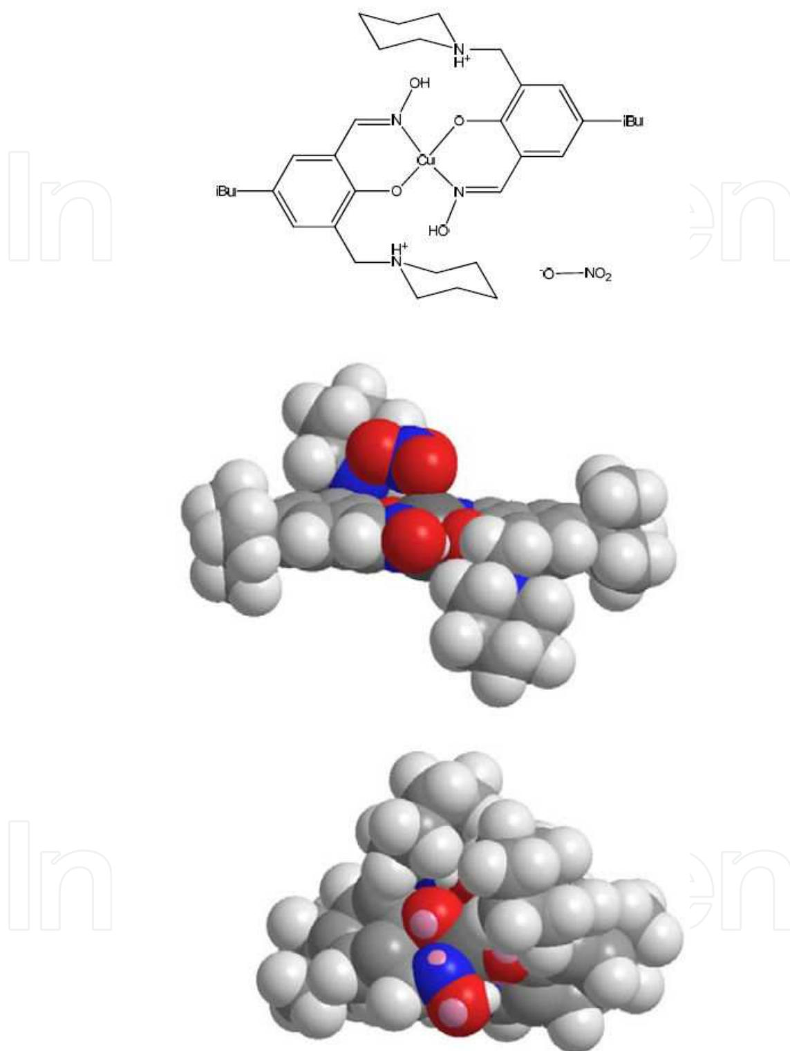
Figure 2. CCDC MIMTOS01 [16]. The compound has a formula C_{34}H_{52}CuN_4O_4^{2+} , 2(NO_3^-) . Novel feature mentioned is that attaching dialkylaminomethyl arms to commercial phenolic oxime copper extractants yields reagents which transport base metal salt very efficiently by forming neutral 1:1 or 1:2 complexes with zwitterionic forms of the ligands. Apparently conformational changes were from a square planar geometry to an umbrella form and twist form (about 45 degree).
