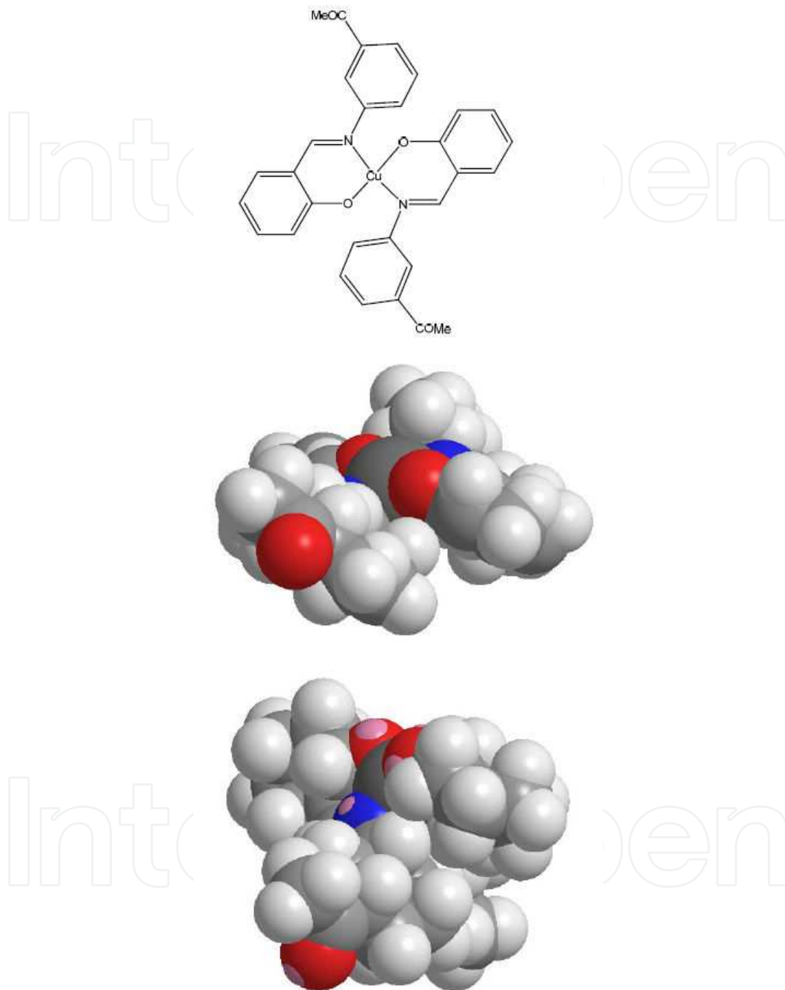
Figure 5. CCDC MIZGIM [19]. The compound has a formula C_{30}H_{24}CuN_2O_4 . Novel feature mentioned is that the coordination geometry around the copper atom in the complex is intermediate between square-planar and tetrahedral with two salicylidimine ligands in trans arrangement. The molecular chains are linked via additional C-H \cdots O hydrogen bonds to form a three-dimensional supramolecular network. Apparently conformational changes were from a moderately umbrella and slightly twist form to a twist (about 90 degree) form.
