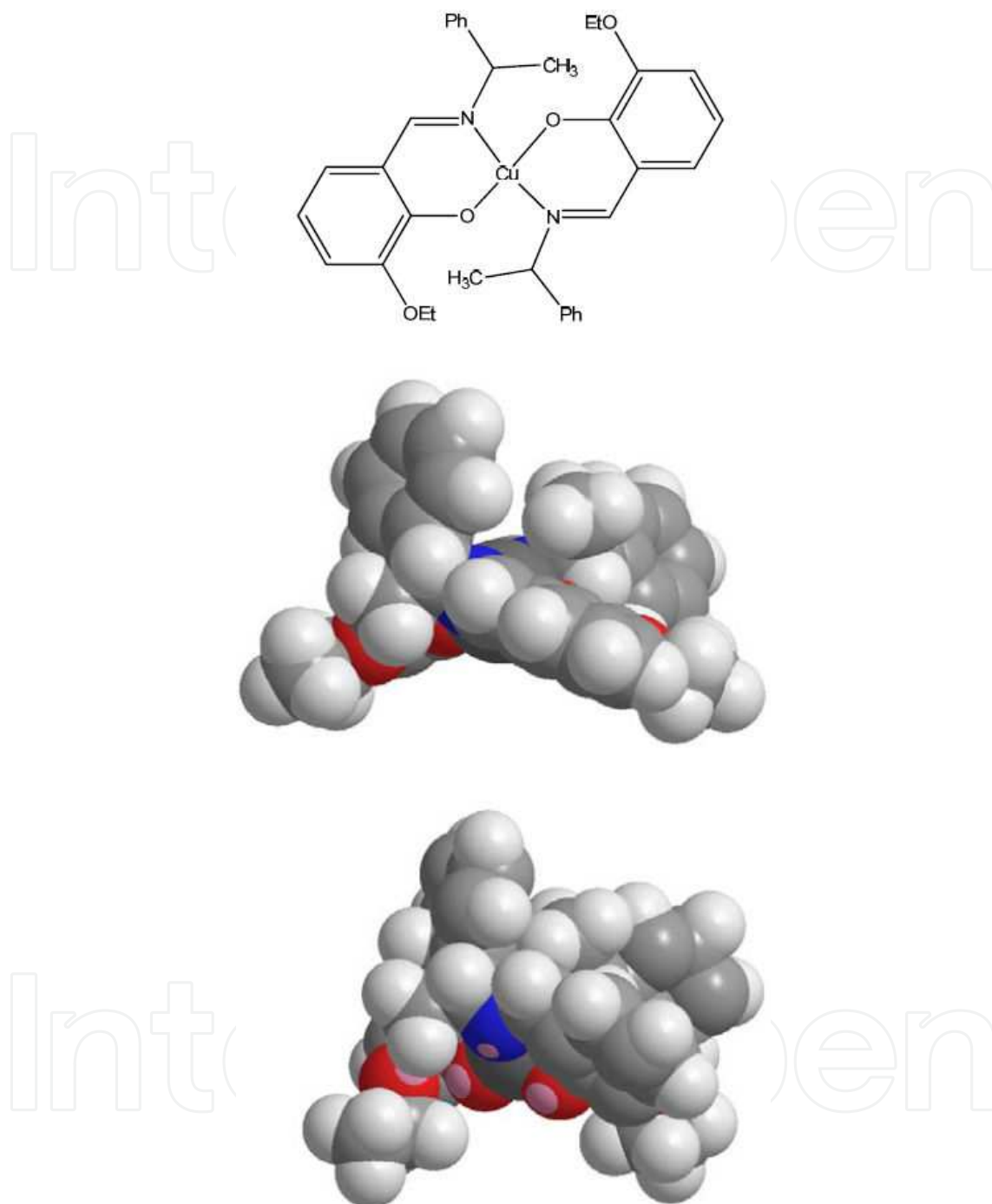
Figure 4. CCDC MAJNIV [18]. The compound has a formula C_{34}H_{36}CuN_2O_4 . Novel feature mentioned is that compressed tetrahedral coordination geometry with an ( R,R )-absolute configuration. These complexes differ from one another with respect to the 1-phenylethylamine moieties, the direction of the benzene rings being inside and outside of the molecules. Apparently conformational changes were from an umbrella and twist (about 45 degree) form to same and twist (about 90 degree) form. The extended conformation of the phenethylimine pendant groups results in crystal packing formed by weakly aggregated planar molecules. Apparently conformational changes were from a relatively flat step form to a significantly sharp step form.
