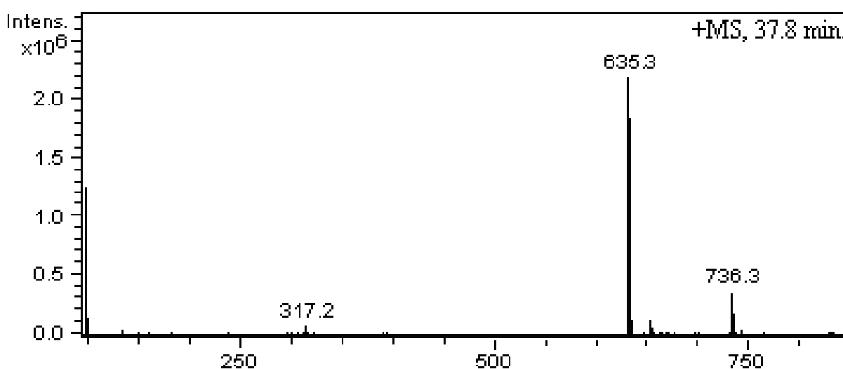
Figure 7. The ESIMS of the Gb-3 eluting at the 37.8 min.
