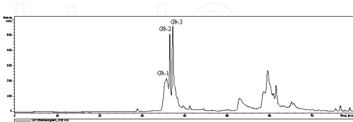
Figure 6. The chromatogram of Ginkgo biloba male autumnal leaves' crude extract. The LC conditions: Column: Nucleosil 100-5 C 4 4x250 mm. The mobile phase: 90% v/v water (0.1% TFA):methanol to 0% v/v water (0.1%TFA):methanol in 80 minutes. Flow rate: 0.2 ml/min. UV detection at \lambda=312 .
