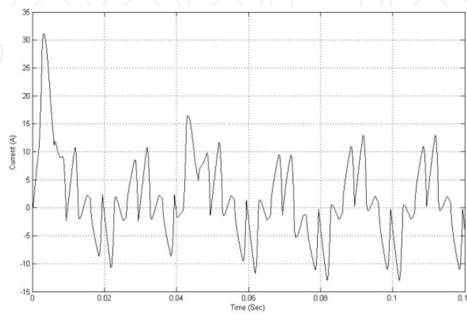
Figure 33. Harmonic current of phase 1
