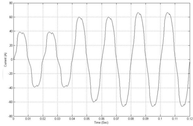
Figure 31. Load side current of phase 1
