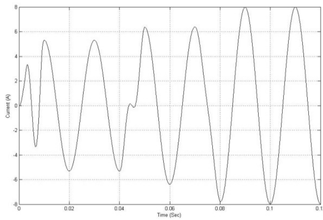
Figure 32. Reactive current of phase 1
