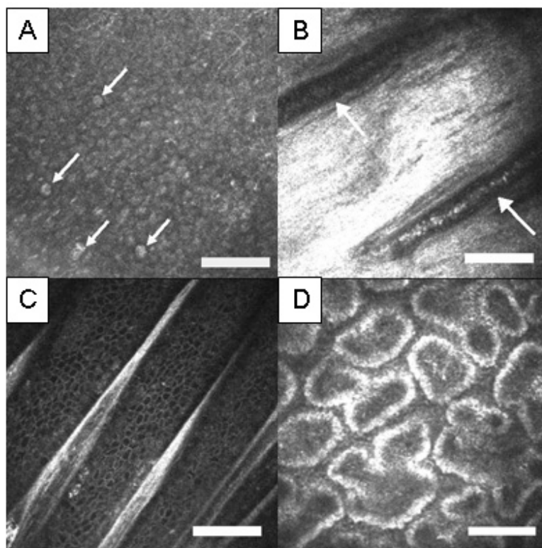
Figure 3. Normal human conjunctiva and meibomian glands. A. Conjunctival epithelium with Goblet cells (arrows). B. Sub-conjunctival fibrous tissue with conjunctival vessels (arrows). C. Palisade of Vogt of corneal limbus. D. Meibomian gland of the upper tarsus. (Bar=100µm)
