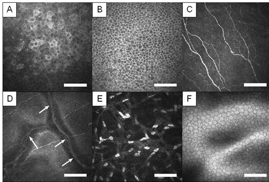
Figure 2. Normal human cornea. A. Superficial epithelial cells. B. Basal epithelial cells. C. Bowman's layer with nerves. D. Bowman's layer with K-structures (arrows). E. Stroma. F. Endothelial cells. (Bar=100µm)
