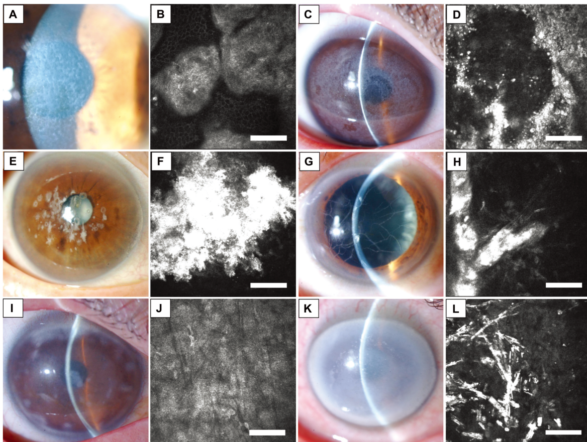
Figure 5. Corneal dystrophies. A. Slit-lamp biomicroscopic photograph of Thiel-Behnke corneal dystrophy ( TGFBI R555Q). Honeycomb-shaped gray opacities were observed at the level of Bowman's layer. B. In vivo laser confocal microscopy showed focal deposition of homogeneous reflective materials with round-shaped edges in the basal epithelial layer. All deposits accompanied dark shadows. C. Slit-lamp biomicroscopic photograph of Reis-Bücklers corneal dystrophy ( TGFBI R124L). Bilateral gray-white, amorphous opacities of various sizes at the level of Bowman's layer were observed. D. In vivo laser confocal microscopy showed focal deposition of highly reflective irregular and granular materials in the basal epithelial layer. No deposits accompanied dark shadows. E. Slit-lamp biomicroscopic photograph of Avellino corneal dystrophy ( TGFBI R124H) showed round gray-white deposits and scattered stellate opacities in the superficial and mid-stroma. F. In vivo laser confocal microscopy showed focal deposits of extremely highly reflective material with irregular edges in the stromal layer. G. Slit-lamp biomicroscopic photograph of lattice corneal dystrophy
