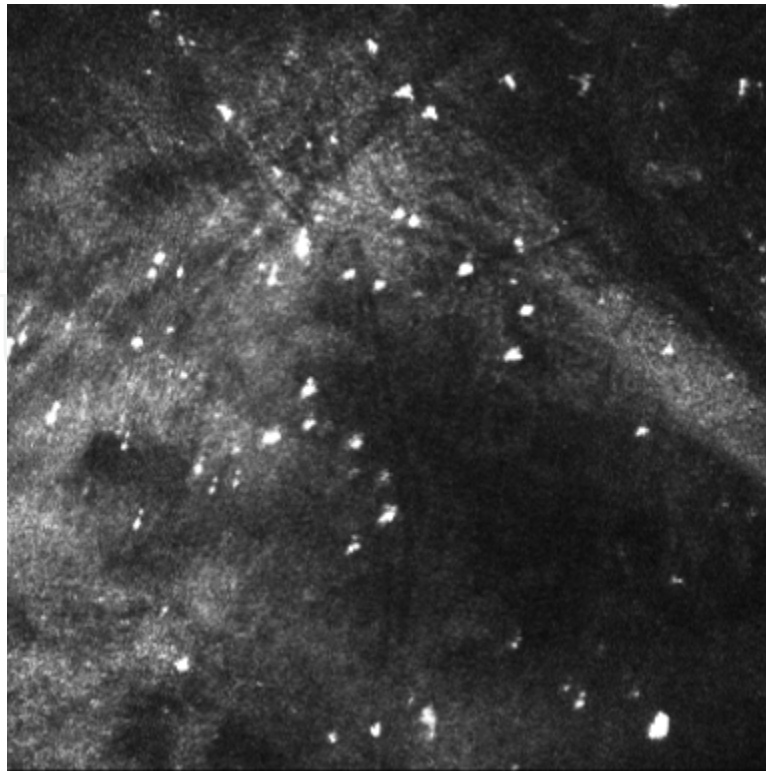
Figure 8. In vivo laser confocal microscopy of donor-recipient interface after DSAEK. At the level of the donor-recipient interface, highly reflective particles and interface haze were observed(400×400μm).
