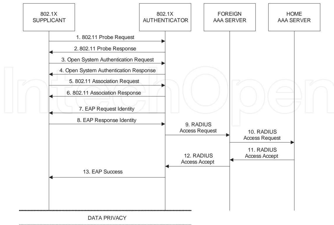
Figure 3. Coordinated authentication message exchange
