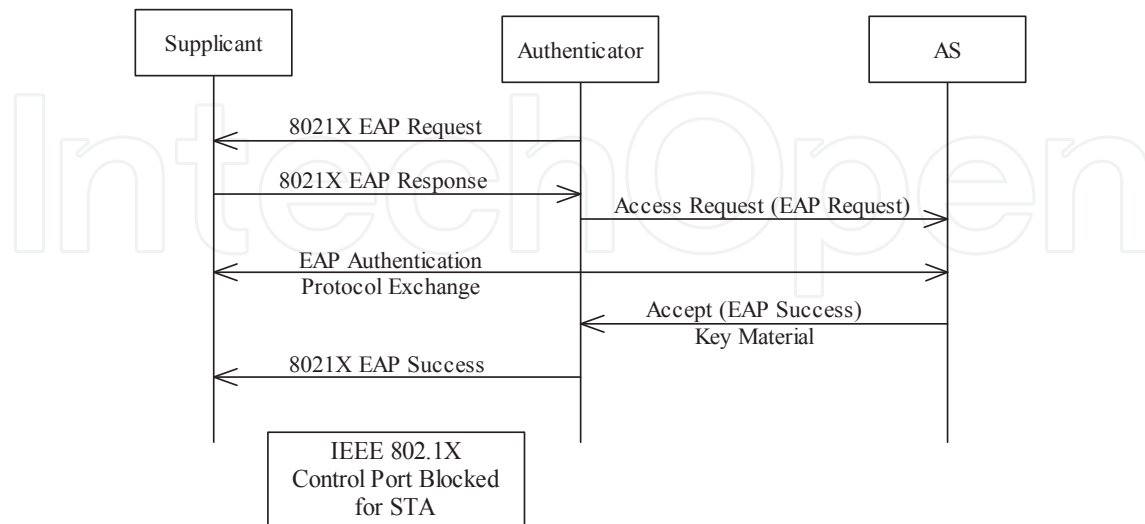
Figure 1. IEEE 802.1X EAP Authentication
