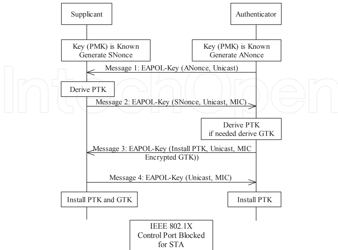
Figure 2. Establishing pairwise & group keys [6]
