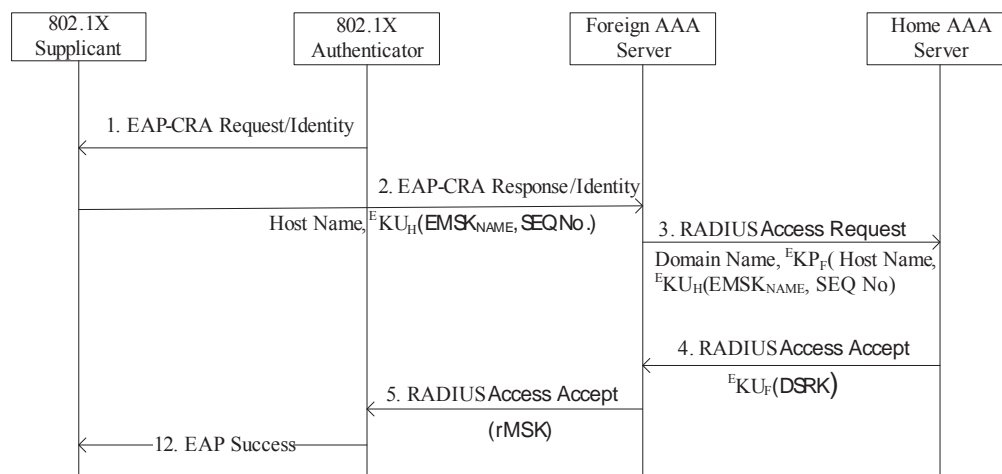
Figure 4. Coordinated Robust Authentication (CRA) Protocol.
