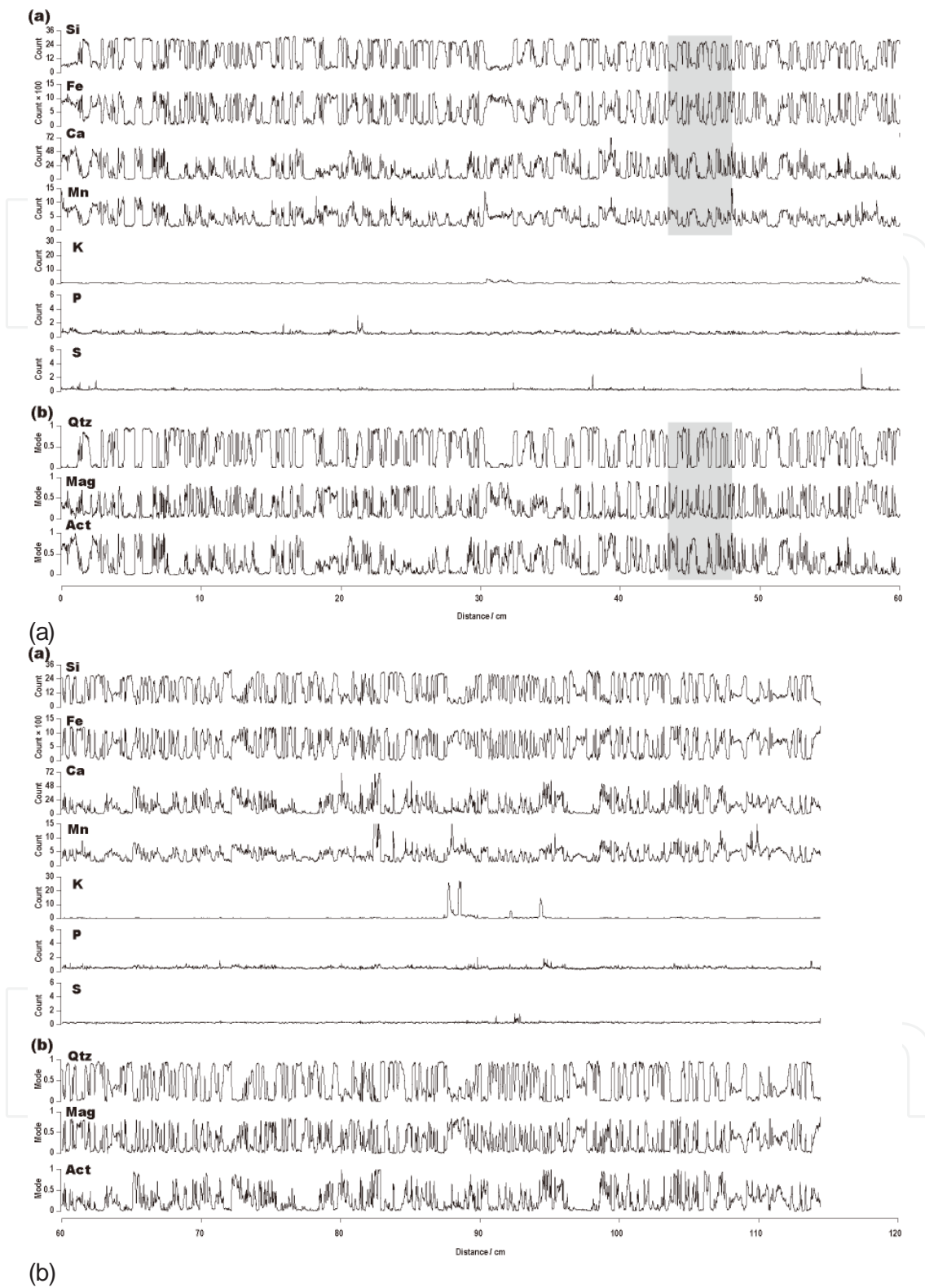
Figure 5. Chemical profiles of the Dwyer Lake BIF samples ( DLS ) in the direction orientated perpendicular to the banded structures. (a) Elemental profiles. The relative abundance of Si, Fe, Ca, Mn, K, P and S are represented by the X-ray photon counts acquired during the micro-XRF analysis. (b) Mineral profiles are calculated from the XRF intensity for Si, Fe, Ca, and Mn. The shaded area corresponds to the XRF images in Fig. 4 and the mineral mode profiles shown in Fig. 7. The abbreviations of the mineral phases follow Kretz [35].
