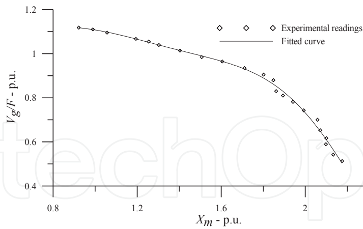
Figure 4. Variation of air gap voltage as a function of magnetizing reactance.
