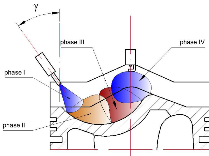
Figure 6. The phases of injected fuel stream
