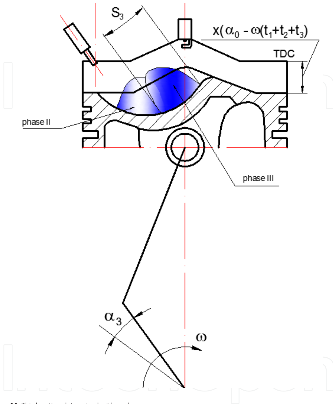
Figure 11. Third section determined with angle \alpha_3
