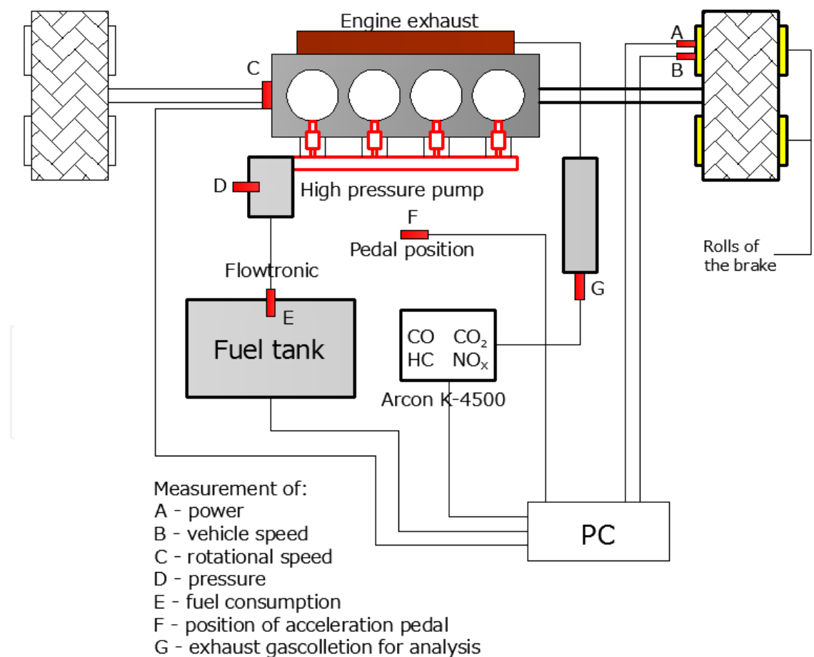
Figure 29. The scheme of the test bed
