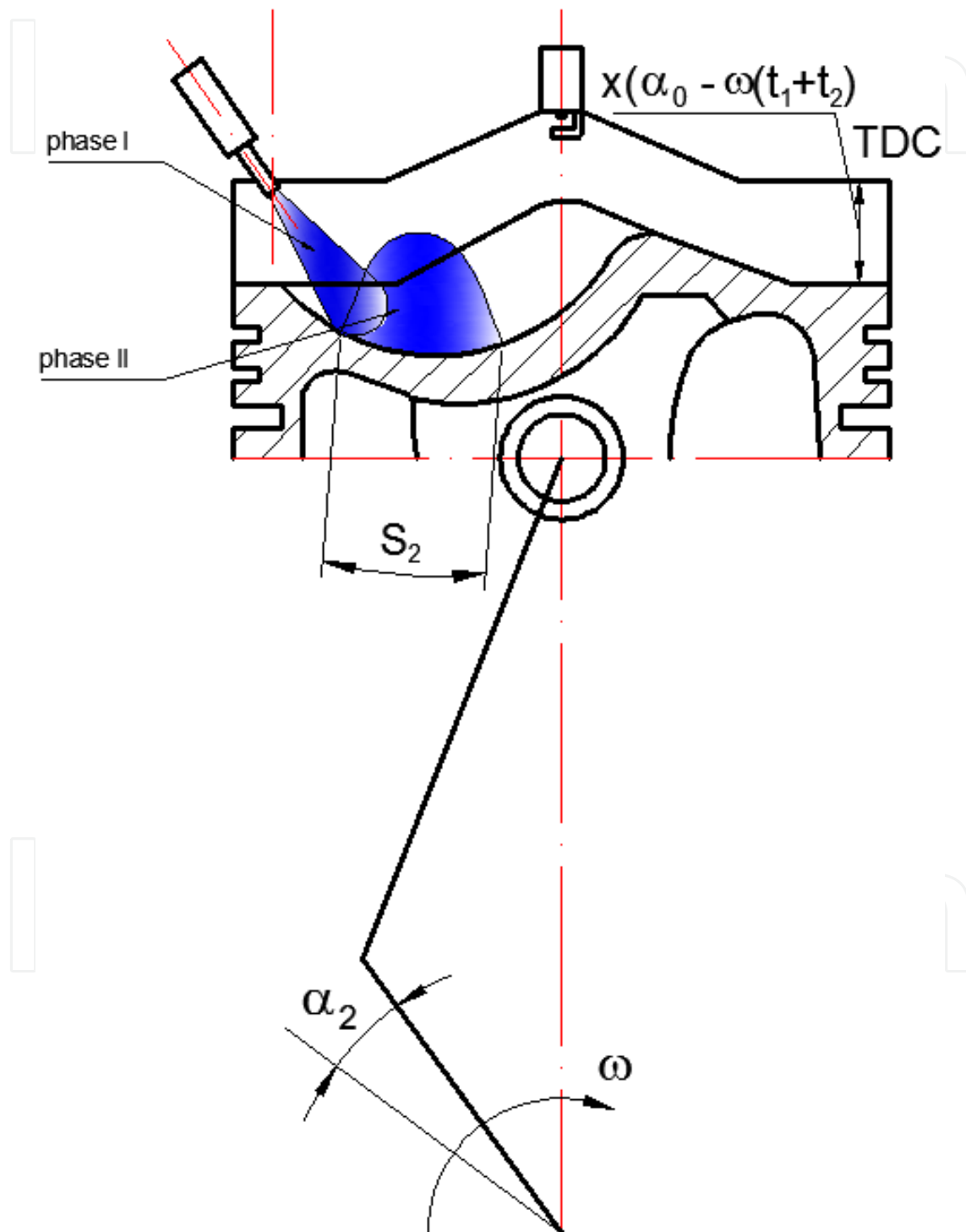
Figure 9. Second section determined with angle \alpha_2
