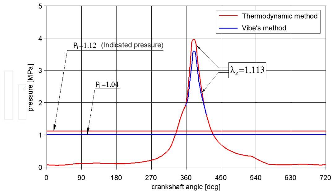
Figure 4. Diagrams of pressures obtained by use of two methods for a substitutive coefficient of air excess \lambda_z = 1.113 and a comparison of indicated pressures calculated by use of the thermodynamic and Vibe's method with indicated pressure in a gasoline direct injection engine
