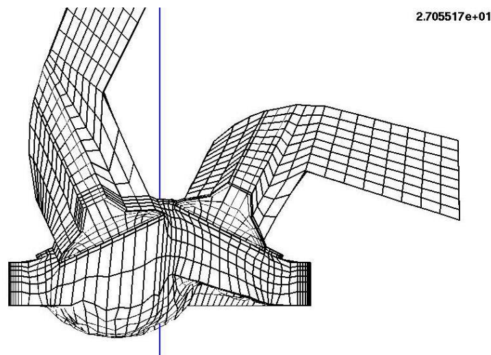
Figure 20. Engine mesh at 27 deg ATDC
