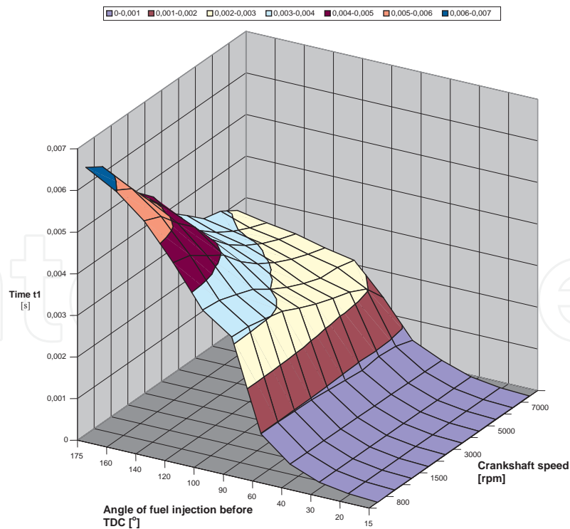
Figure 8. The time which the fuel stream takes to go from the moment of injection to its contact with the piston head, depending on the crank angle and the rotational speed of the engine, at constant injection pressure 5 [MPa]
