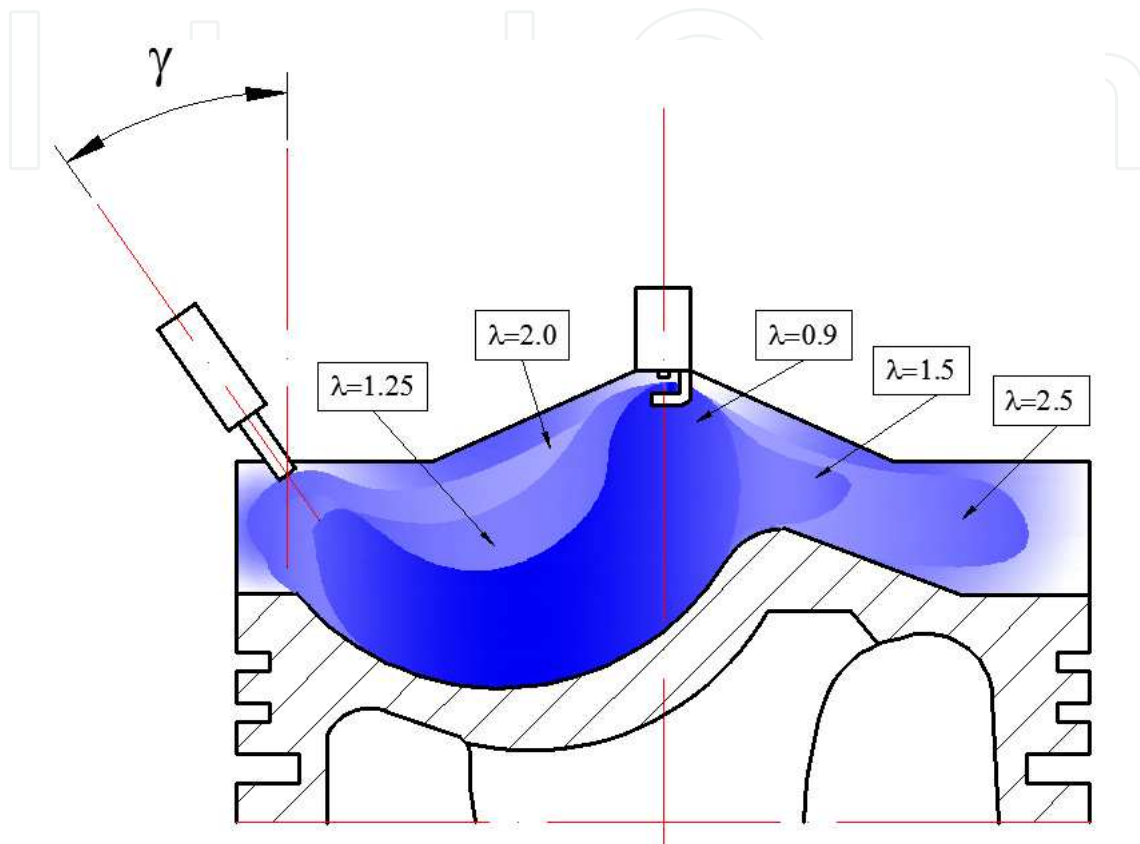
Figure 1. Variation of fuel mixture in combustion chamber.
