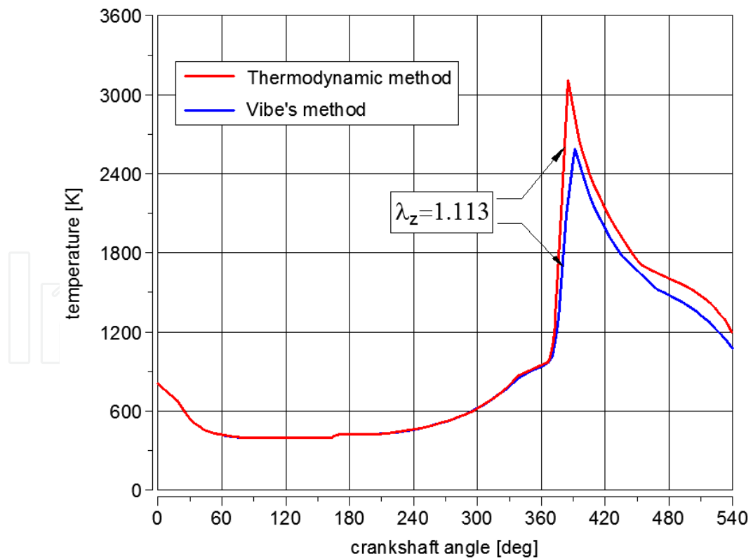
Figure 5. Diagrams of temperature obtained by use of two methods for a substitutive coefficient of air excess \lambda_z = 1.113
