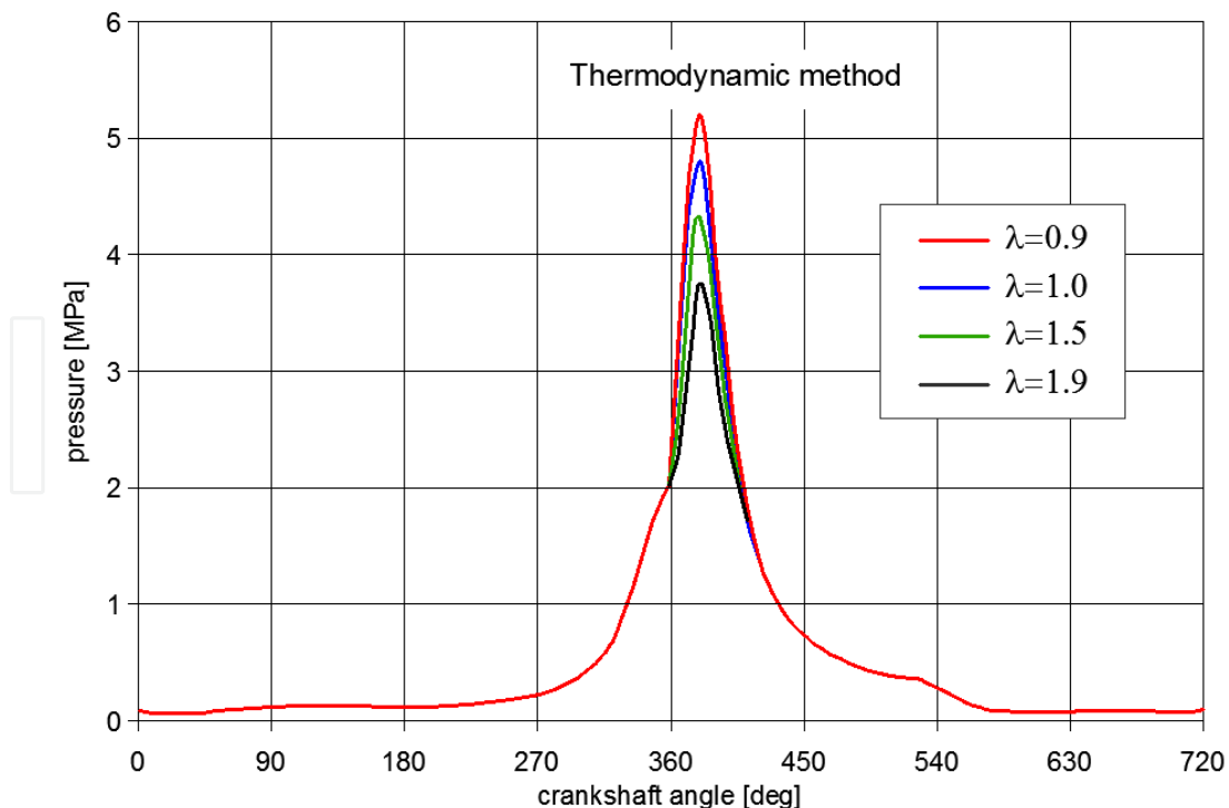
Figure 2. Traces of pressure changes in the cylinder for various coefficient of air excess \lambda obtained by use of the thermodynamic method
