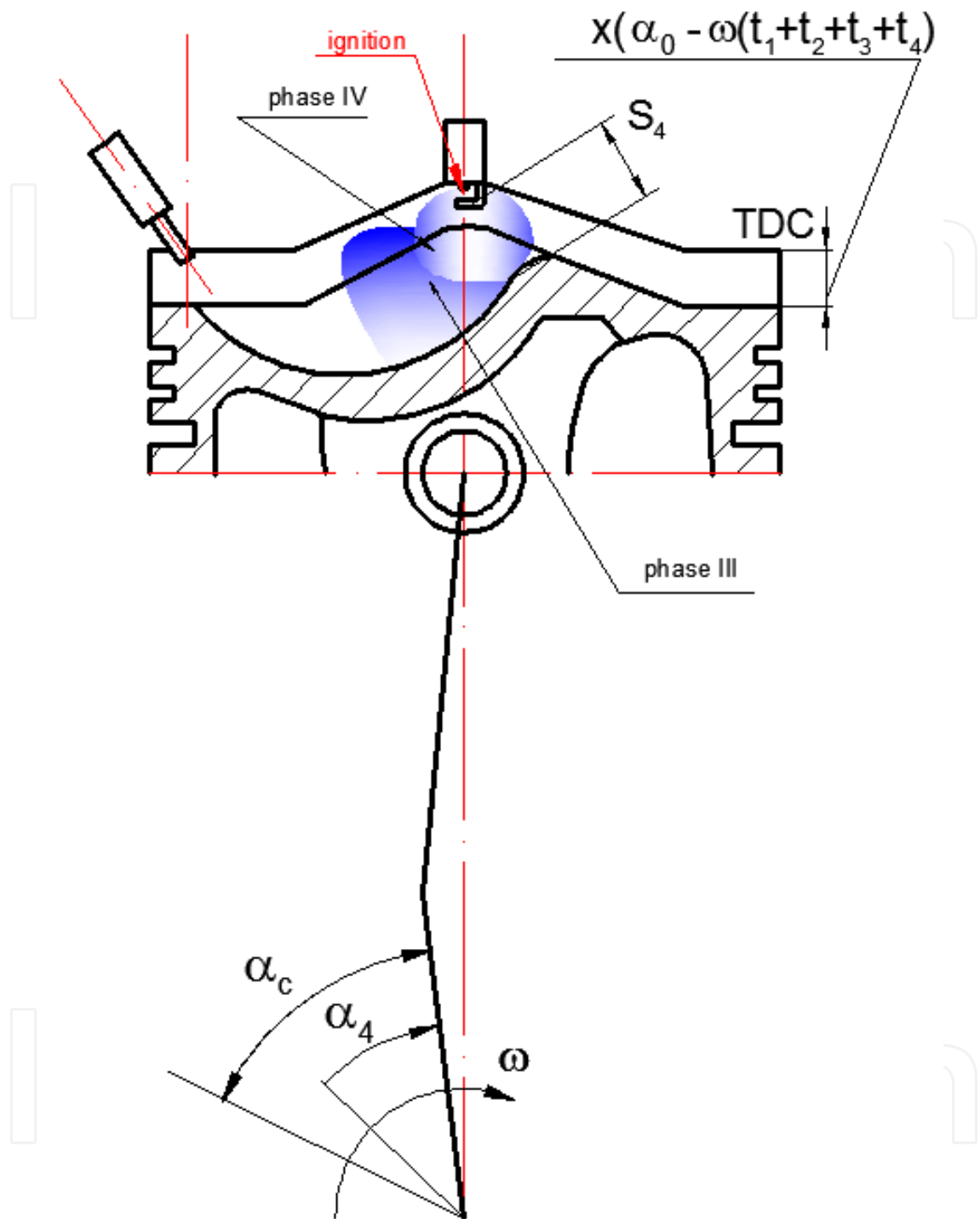
Figure 13. The fourth sector – fuel mixture reaches the electrodes of the spark plug; it is determined with angle \alpha_4
