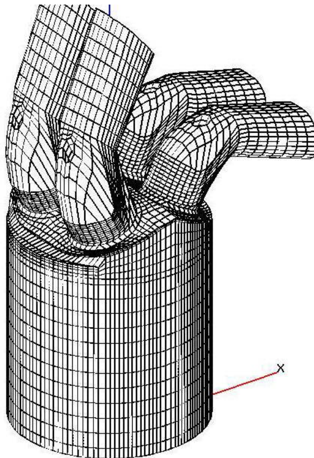
Figure 18. Complex mesh of Mitsubishi GDI engine
