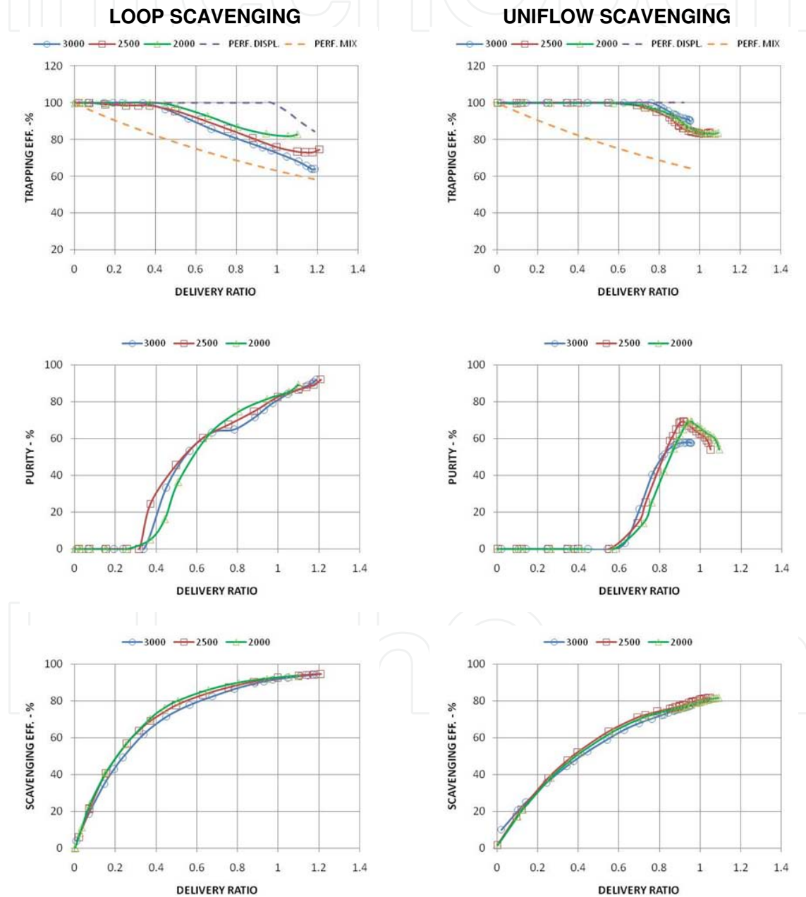
Figure 6. Trapping efficiency, Purity and Scavenging efficiency plotted as a function of Delivery Ratio. Values calculated at three different operating conditions on the optimized Loop and Uniflow configurations (engine speed: 2000, 2500 and 3000 rev/'), reference [14]
