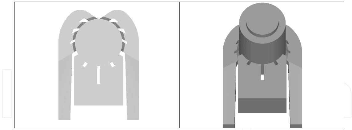
Figure 3. Schematic of intake and exhaust ports in the Loop configuration#2
