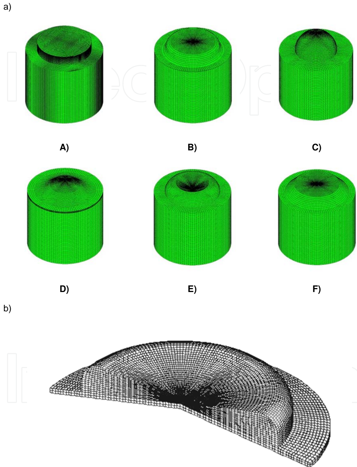
Figure 9. a): The analyzed combustion chamber grids at EPO/EPC for the automobile engine: A) Cylindrical; B) Smoothed Cylindrical; C) Spherical; D) Smoothed Spherical; E) Reverse Bowl; F) Conical. For details, see [8, 20].b): Chamber optimized for an aircraft engine [13, 14]
