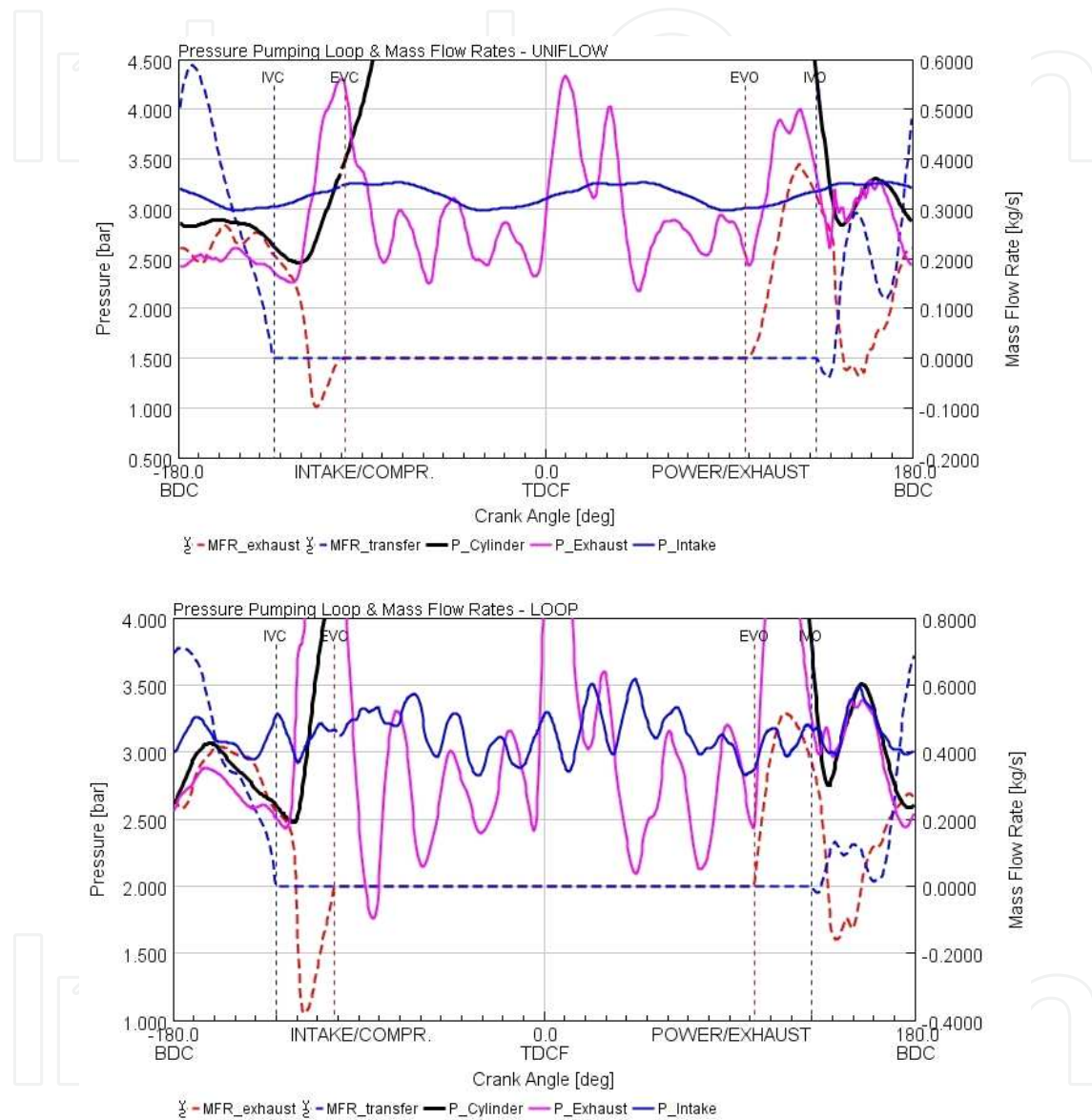
Figure 15. Pumping loop and mass flow rates at 2600 rpm, full load, calculated for the two types of aircraft engines described in [13]
