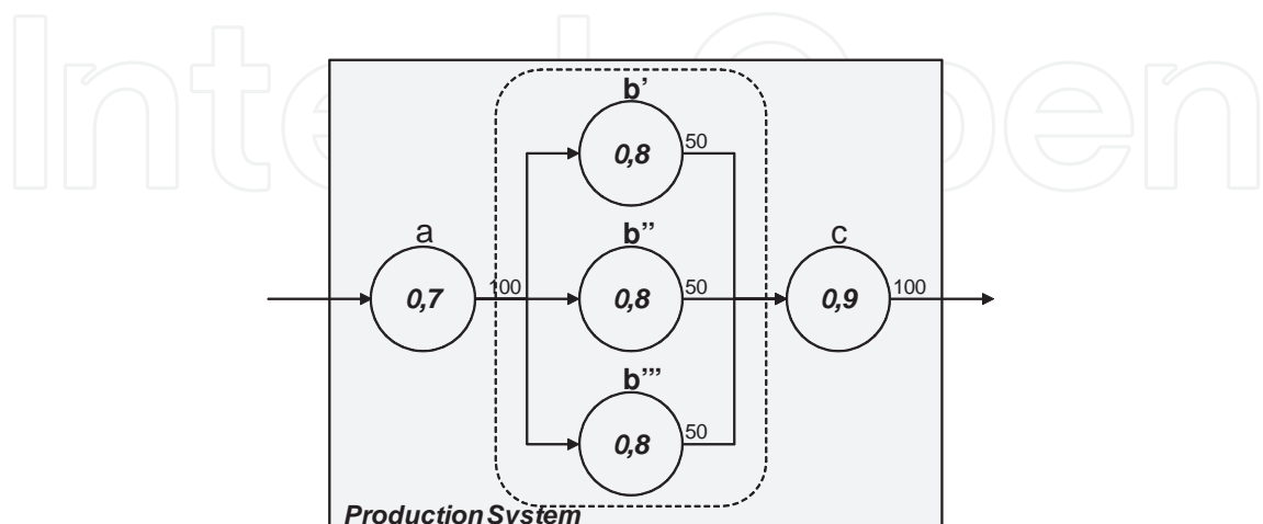
Figure 8. Availability of partially redundant equipments connected with not redundant equipments
