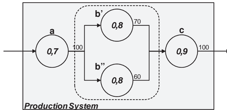
Figure 9. Availability of partially redundant equipments connected with not redundant equipments at modular capacity
