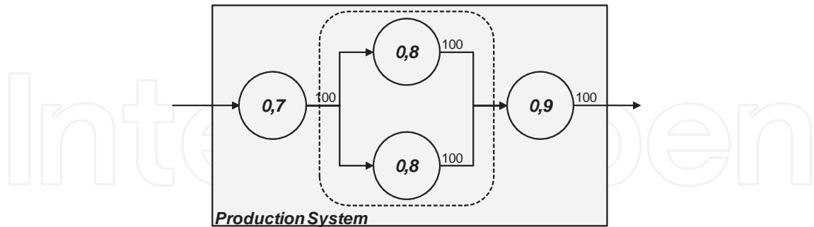
Figure 7. Availability of totally redundant equipments connected with not redundant equipments
