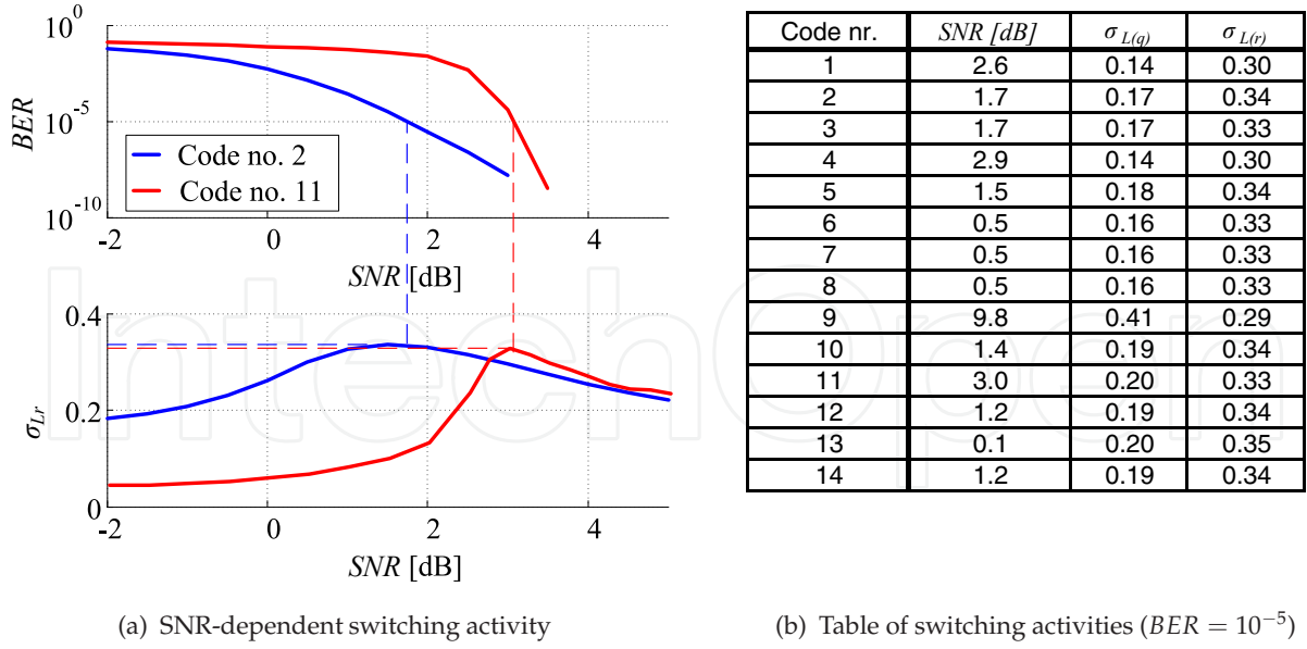
Figure 18. Switching activity
