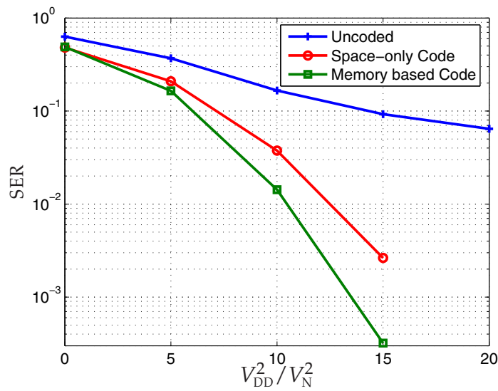
Figure 13. Symbol error rate (SER) as function of V_{DD}^2/V_N^2 for an interconnect with four lines, employing a memory-based code of rate 3/4, compared to the uncoded case. The performance of a space-only code is also plotted.
