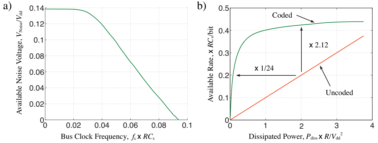
Figure 4. a) Maximum permissible noise-voltage at the receiver of a four-conductor bus as function of the bus clock frequency, b) achievable information rates of coded and uncoded transmission as function of the dissipated power [7].
