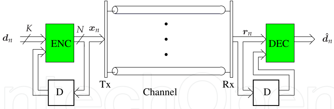
Figure 12. Noisy bus communication with a memory-based Code.
