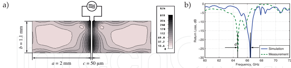
Figure 7. (a) Top view and current distribution of a two-patch dipole antenna, operating at 66 GHz, (b) Measured return loss of the on-chip open slot antenna [14, 15].
