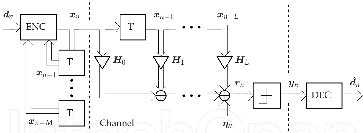
Figure 11. Encoding and Decoding for MIMO Channels with ISI and Single-Bit Output Quantization.
