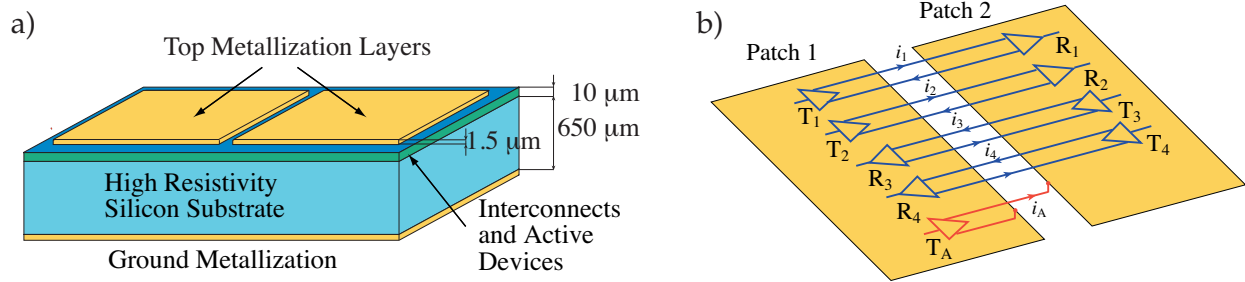
Figure 5. a) Schematic drawing of a chip with an integrated antenna, b) Differential lines, connecting the digital circuits under the separate antenna patches.
