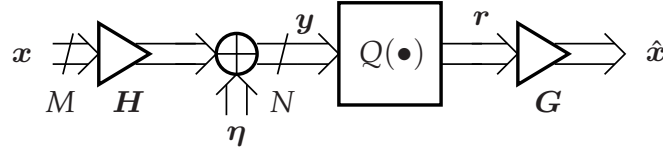
Figure 14. Quantized MIMO System.
