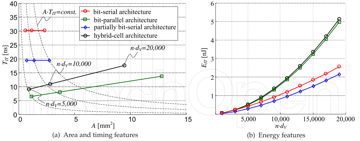
Figure 23. Comparison of area, timing and energy features ( d_V = 6, d_C = 32, M_R = 4, w = 6, \lambda = 40\text{nm} )
