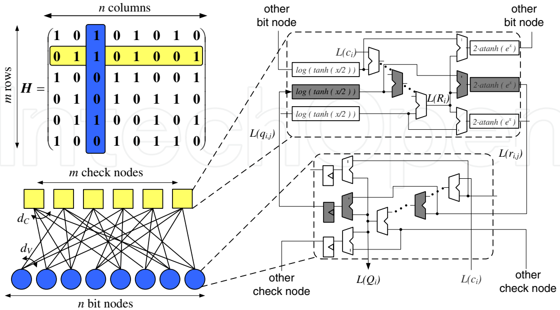
Figure 16. Parity-check matrix, Tanner-Graph and non-linear recursive decoder loop
