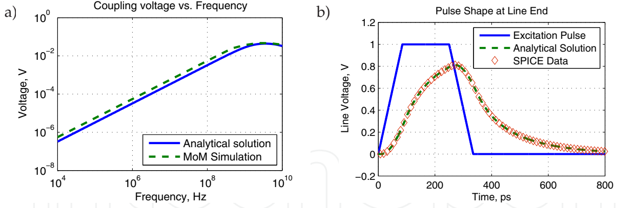
Figure 3. a) Frequency response of the crosstalk voltage at the end of the line, b) pulse response at the end of the line [18].
