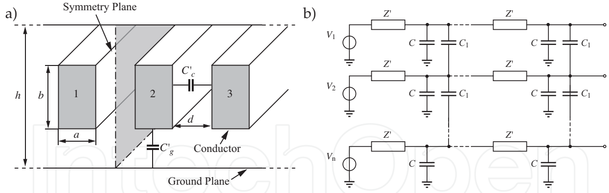
Figure 1. a) A cross section of three-wire digital bus with a coupling and a ground capacitance [10] and b) equivalent lumped element circuit [8].
