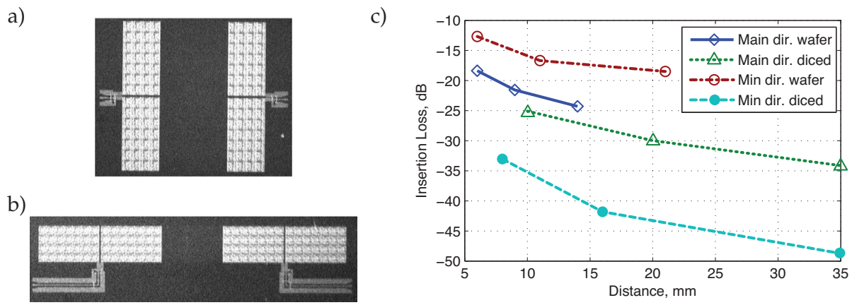
Figure 8. Antenna orientation with a) collinear and b) parallel slots, c) Measured insertion loss of a wireless chip-to-chip link depending [14, 15].
