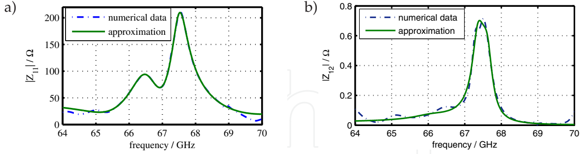
Figure 9. Comparison of the numerical data of (a) |Z_{11}| and (b) |Z_{12}| obtained from the full-wave simulation of the wireless transmission link with the data computed from lumped element model
