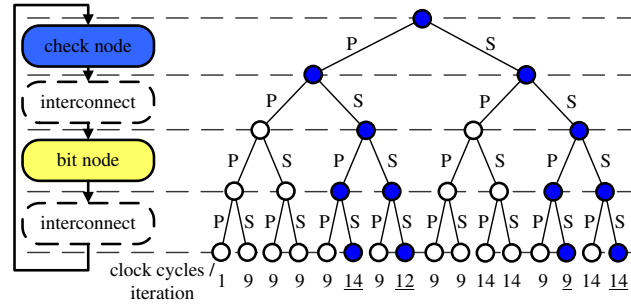
Figure 21. Bit- and check-node architecture design space.
