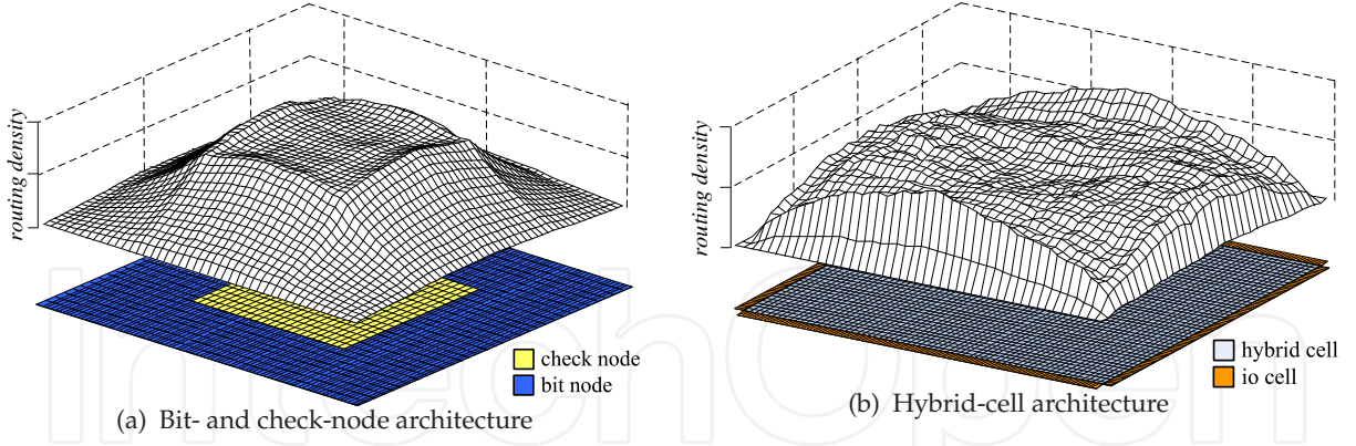
Figure 20. Routing density
