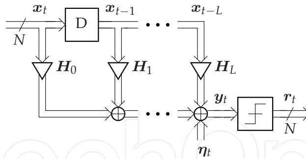
Figure 10. MIMO channel with ISI and single-bit outputs modeling wired as well as the wireless interconnects.
