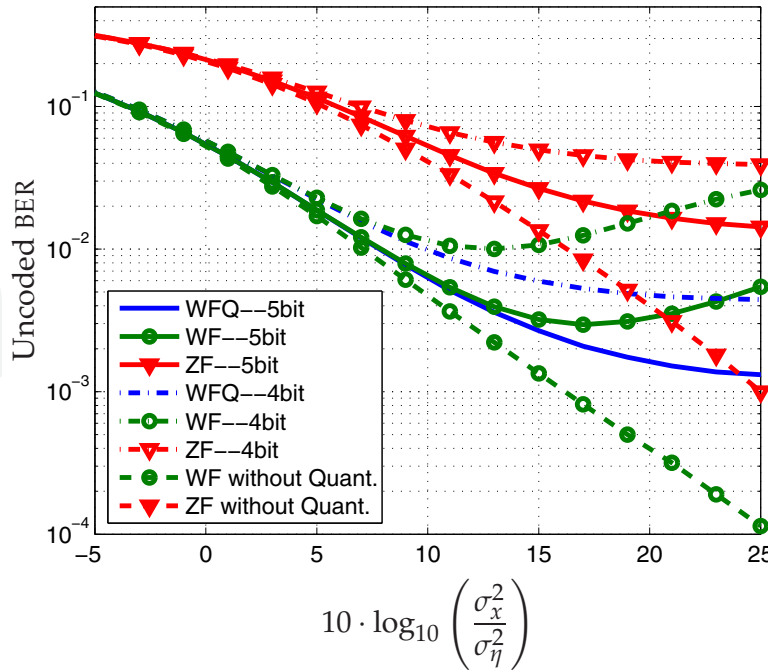
Figure 15. The WFQ vs. the conventional WF and ZF receivers, QPSK modulation with M = 10 , N = 10 , 4- ( \rho_q = 0.01154 ) and 5- ( \rho_q = 0.00349 ) bit uniform quantizer.
