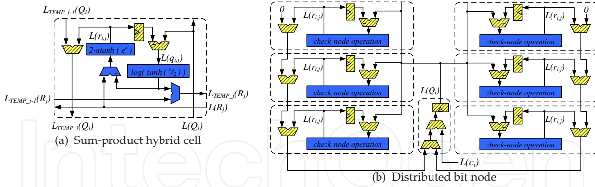
Figure 19. Hybrid-cell decoder architecture
