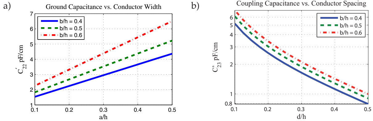
Figure 2. a) Ground capacitance vs. geometry for digital transmission line, filled in with Si, d/h = 0.125 , b) Coupling capacitance vs. geometry for digital transmission line, filled in with Si, a/h = 0.25 [10].
