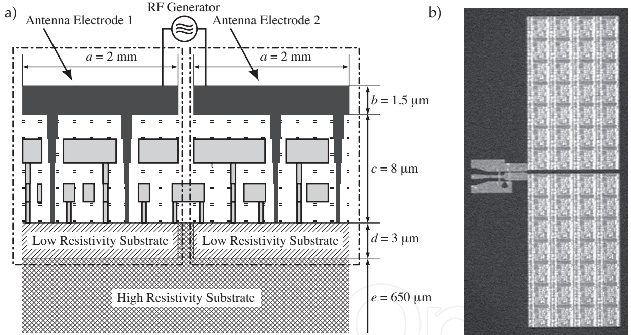
Figure 6. Cross-sectional view of integrated on-chip antenna, using the ground planes as antenna electrodes [11, 14].
