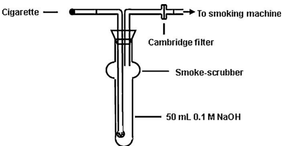
Figure 10. Schematic diagram of solution absorption method [24].
