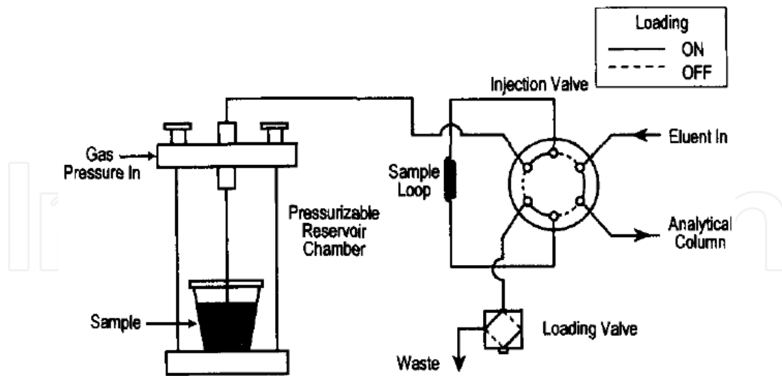
Figure 8. IC system configuration for direct-injection sample loading [21].
