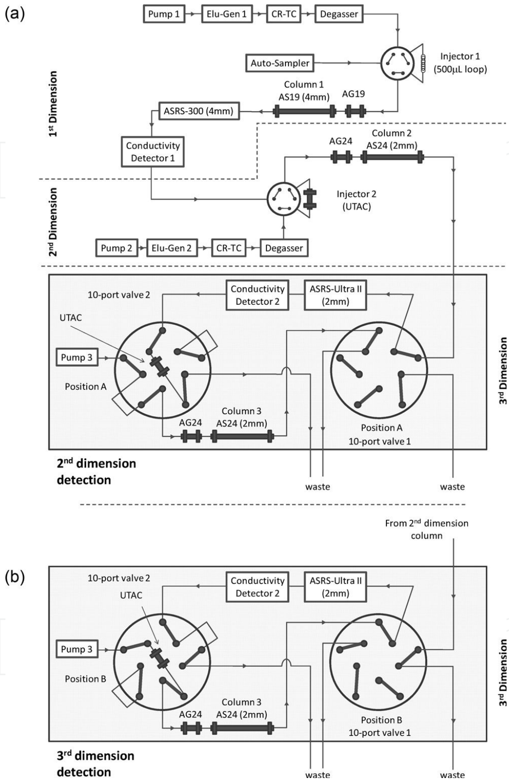
Figure 6. Schematic diagram of instrumentation used to perform the multi-dimensional IC. (a) 10-Port valve positions for detection of 2 nd dimension separation (i.e. effluent from column 2 diverted through conductivity detector 2). (b) 10-Port valve positions for injection of 2 nd dimension cut fractions onto 3 rd dimension column with subsequent detection using conductivity detector 2 [12].
