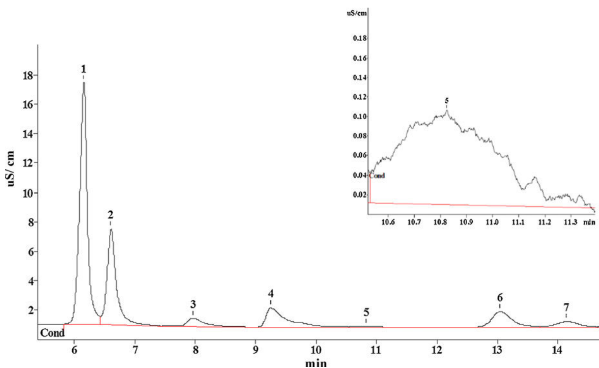
Figure 14. Chromatogram of smog chamber filter analysis from reaction of trimethylamine with ozone. Analytes: 1- sodium, 2-ammonium, 3-potassium, 4-dimethylamine ( 1.72 \mu\text{g}/\text{m}^3 ), 5-trimethylamine-N-oxide ( 0.25 \mu\text{g}/\text{m}^3 ), 6-magnesium, and 7- trimethylamine ( 0.57 \mu\text{g}/\text{m}^3 ). The inset is a magnification of the trimethylamine-N-oxide peak (5) from the chromatogram [27].
