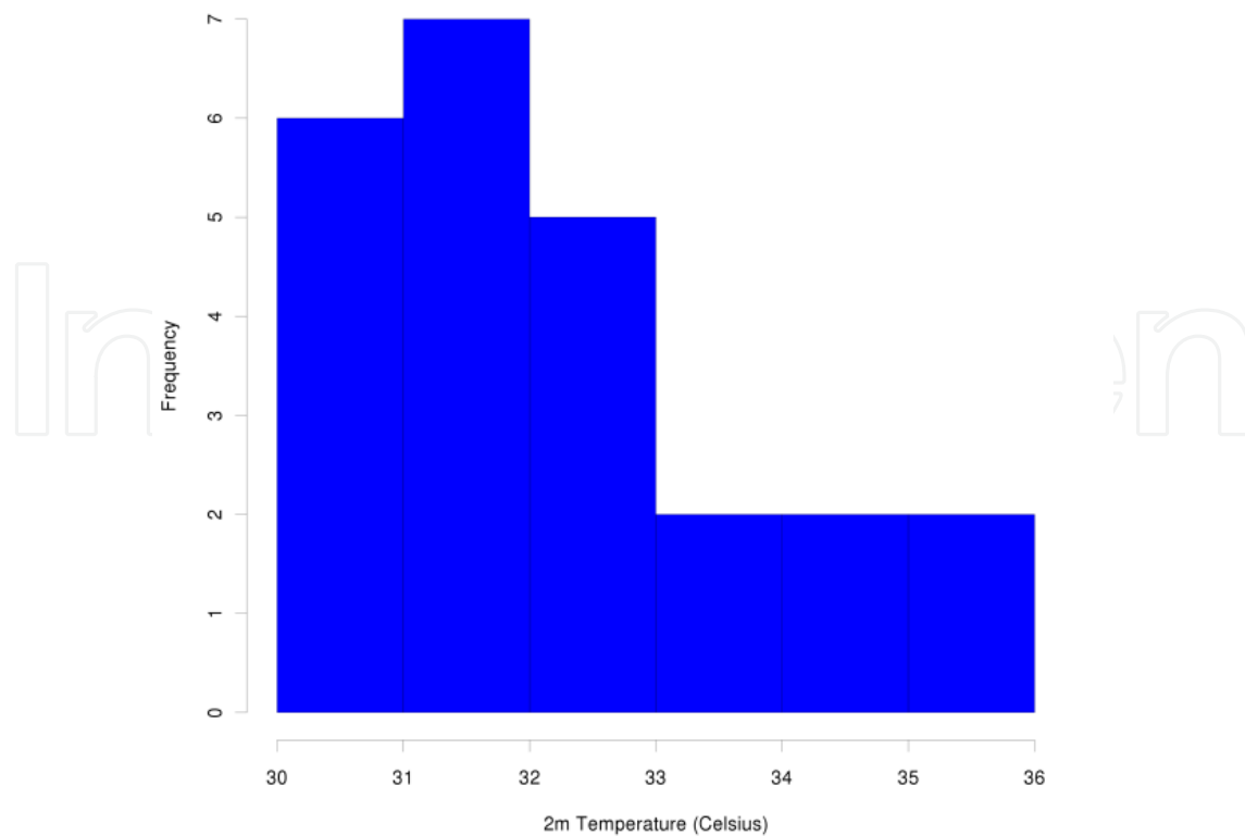
Figure 7. Histogram of 2m Temperature. AEMET-SREPS H+60 predicted values at the grid point closest to Seville. Valid time: 30 th June 2011, 12 UTC.
