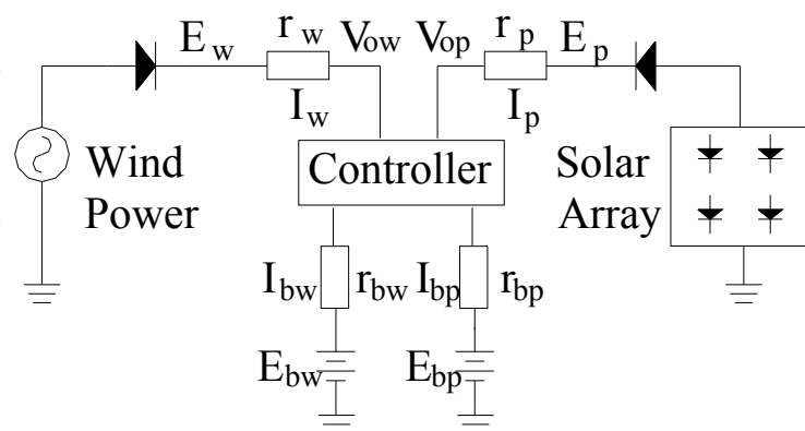
Figure 5. Microprocessor-controlled wind and PV energy charging system. Both power sources charge the two batteries. According to the wind and solar energy conditions, the controller regulates the charging conditions for E_{bw} and E_{bp} . There is no power loss in this charging system. When there is only one power source, it can charge both batteries. With both power sources and high wind energy, the excess wind energy charges battery E_{bp} . The controller improves greatly the reliability of this charging system.
