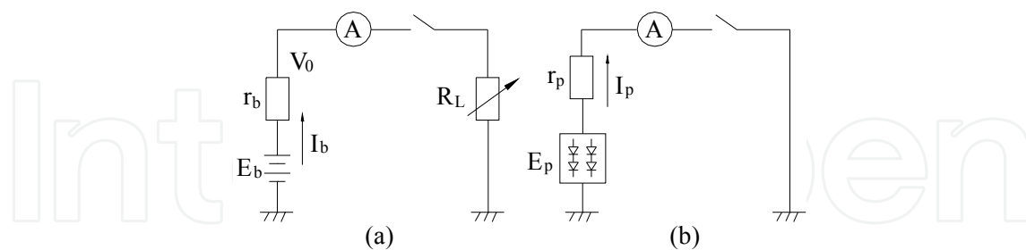
Figure 6. (a) Circuit for measuring battery source resistance. Because much energy is stored in the battery E_b and the battery source resistance r_b is small, R_L is employed to limit the discharging current I_b . (b) Circuit for measuring solar cell internal resistance. Solar current I_p is varied by adjusting the orientation of the solar cell panel relative to the sun.
