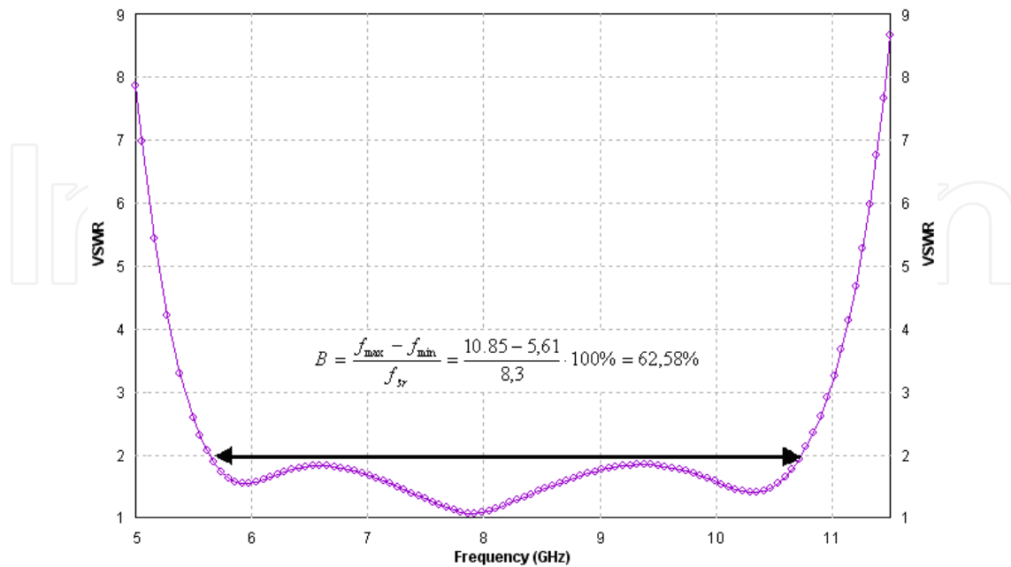
Figure 7. VSWR of optimal single patch antenna.
