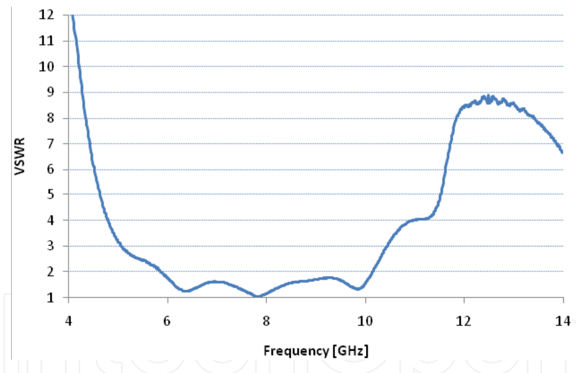
Figure 17. Measured VSWR of optimal single patch.
