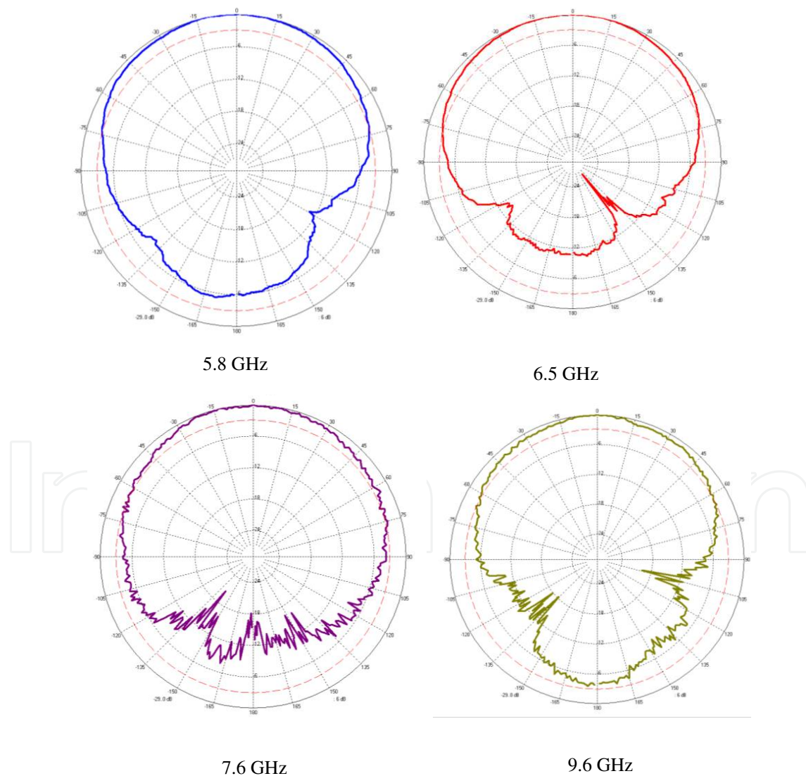
Figure 20. Radiation patterns(H - plane).
