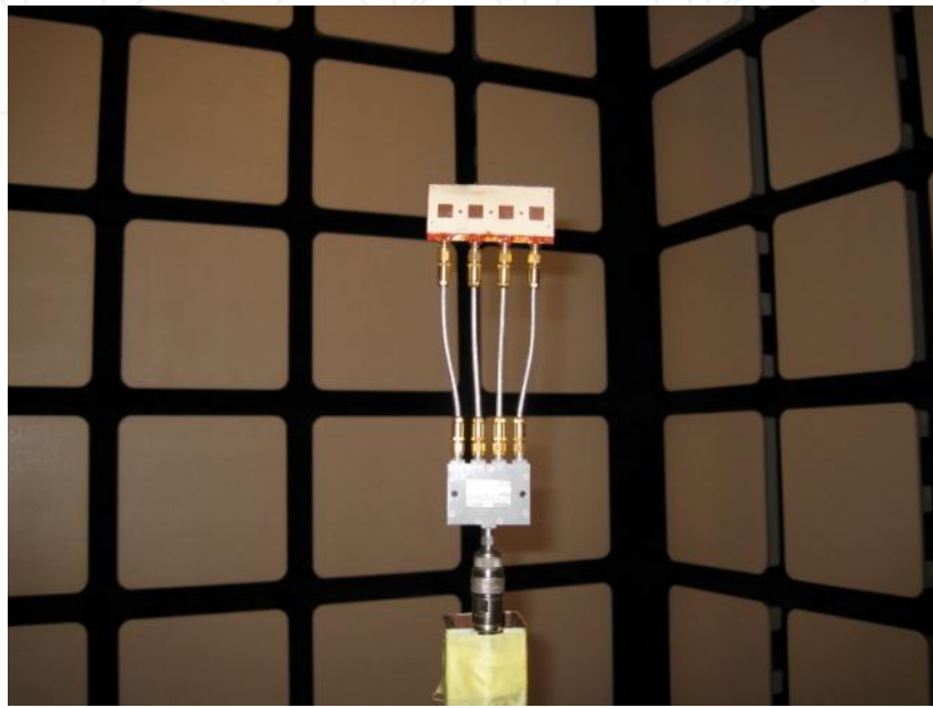
Figure 23. Antenna array during measurements in anechoic chamber.
