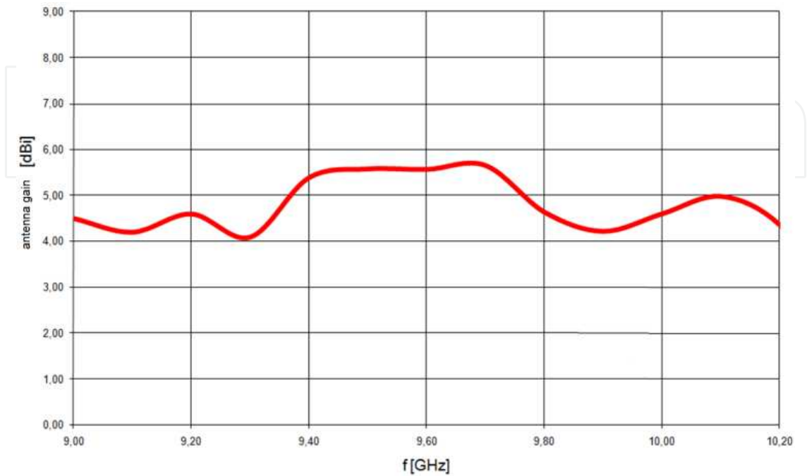
Figure 21. Measured antenna gain versus frequency.
