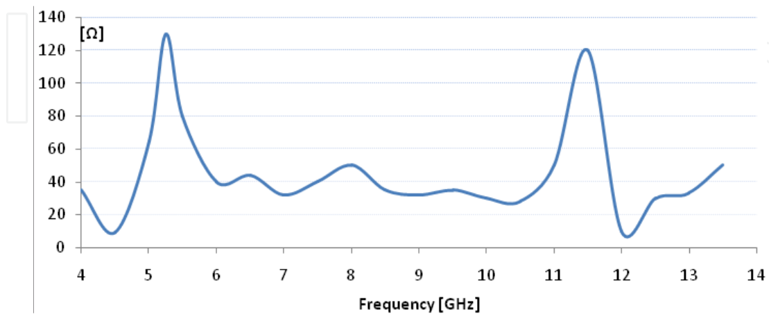
Figure 24. Impedance of antenna array- measurements.
