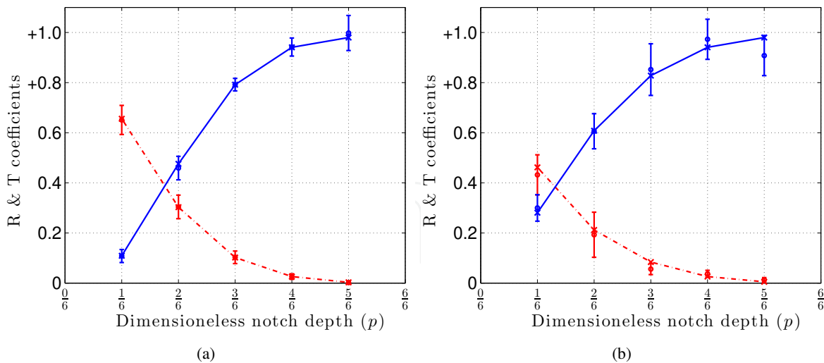
Figure 16. Comparison between numerical and experimental results of the power reflection (---) and transmission (—) coefficients of the modes A_0 (a) and S_0 (b) when they are launched and interact with symmetrical notches.
