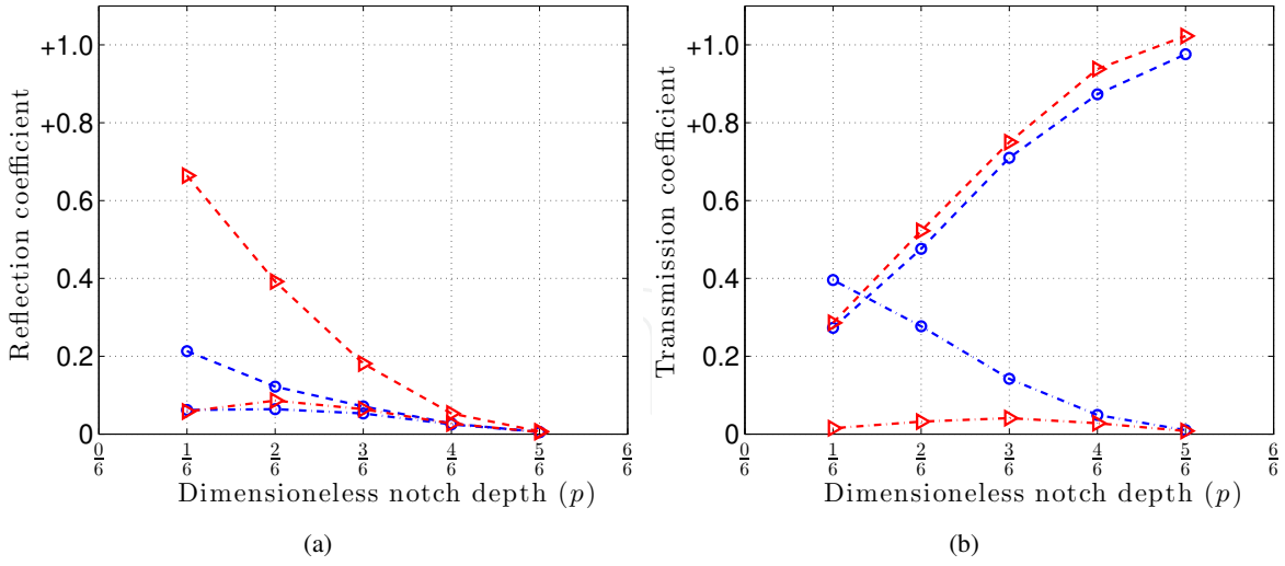
Figure 14. Comparison between the power reflection (a) and the transmission (b) coefficients of the A_0 (---) and S_0 (---) modes computed for an asymmetric step down ( \blacktriangleright ) and step up ( \circ ) when the S_0 mode is launched.
