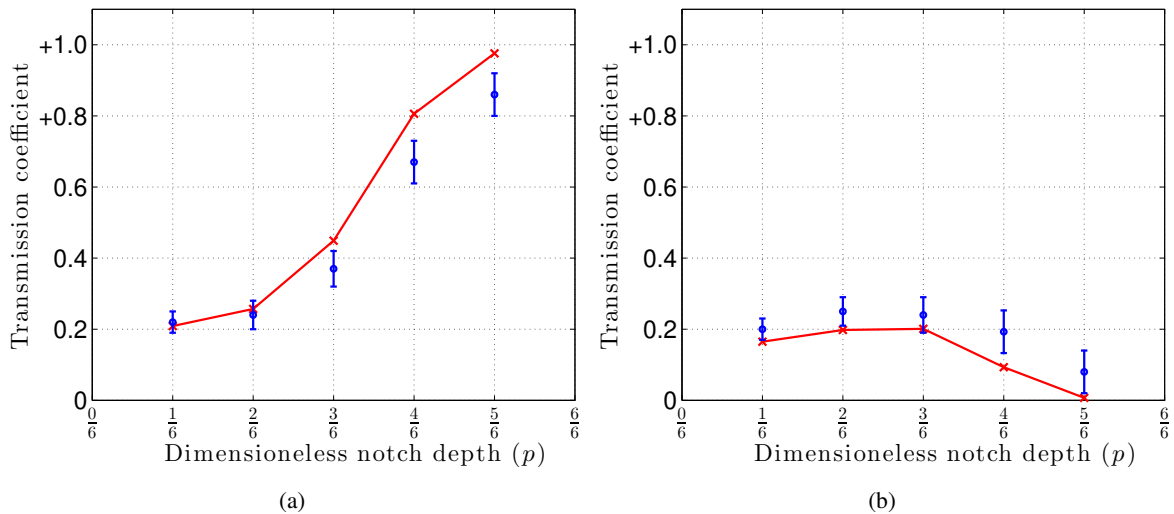
Figure 18. Comparison between numerical (—) and experimental (•) results of the power transmission coefficients of the A_0 (a) and S_0 (b) modes when the A_0 mode is launched and interacts with asymmetrical notches.
