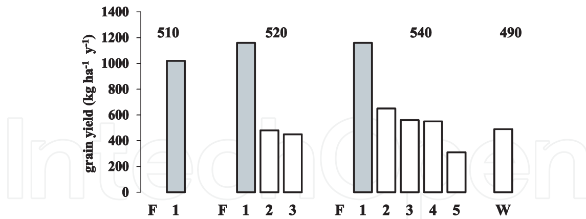
Figure 10. Grain yield (1994-2000) of spring wheat affected by distance from fallowing year. (F is fallow; 1, 2, 3...5 are succession of crops after fallow. (the numbers above bars are average yield per rotation including the fallow year).
