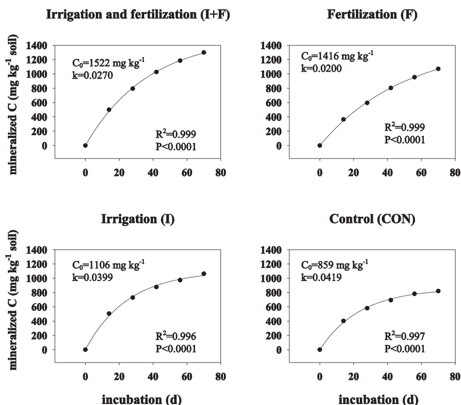
Figure 7. Fitting curves of carbon mineralization in fertilization experiment, Kherson, as described by the first order kinetic model: C_{min} = C_0(1 - e^{-kt}) , where C_{min} is the mineralized C at time t , C_0 is the potentially mineralizable C (PMC), k is the mineralization rate constant
