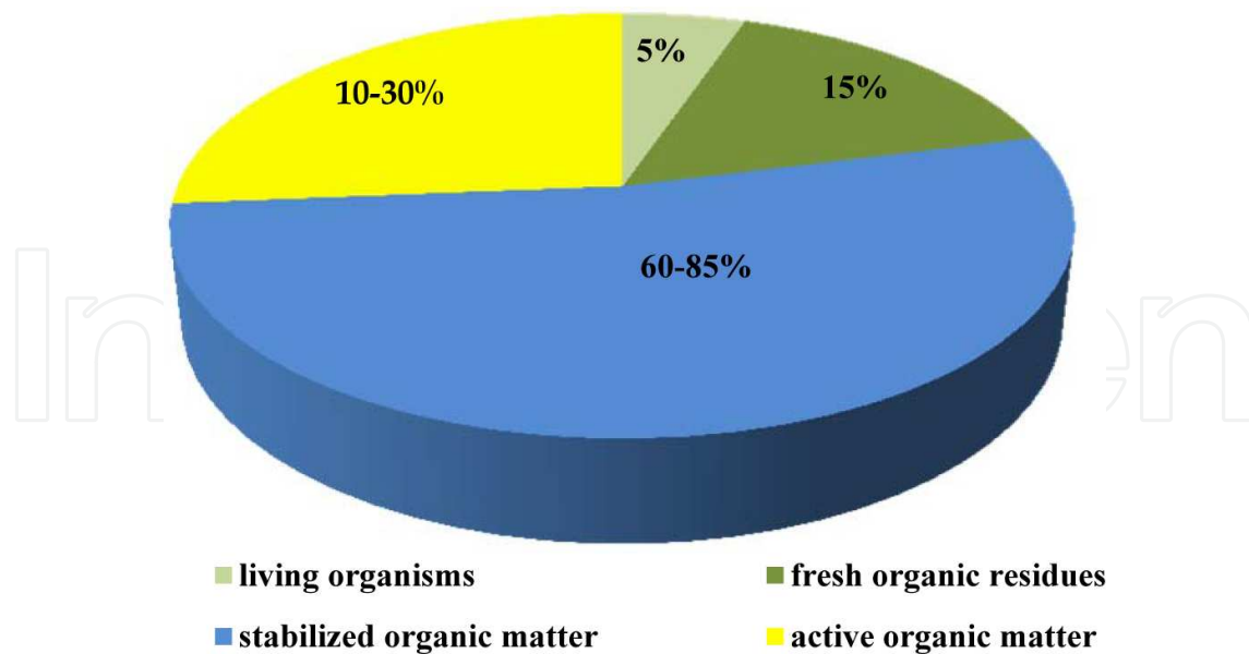
Figure 2. Composition and distribution of fractions of soil organic matter
