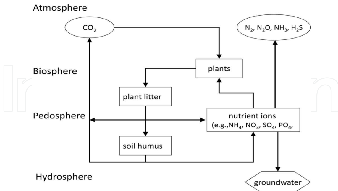
Figure 1. Conceptual model of soil organic matter decomposition (modified from [106])
