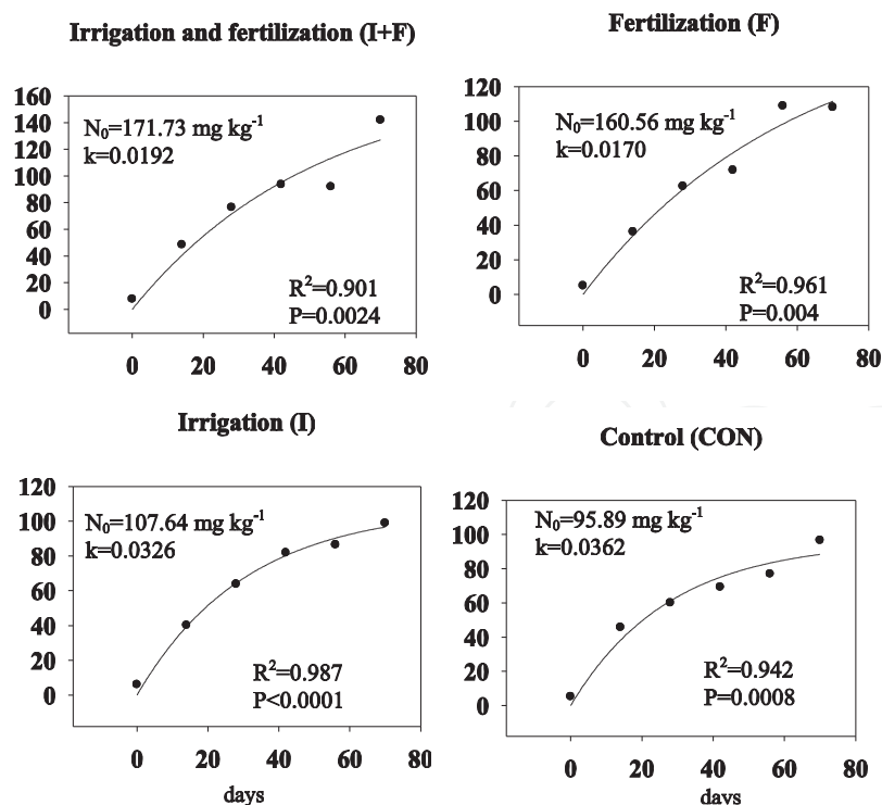
Figure 6. Fitting curves of nitrogen mineralization in fertilization experiment, Kherson, as described by the first order kinetic model: N_{min} = N_0(1 - e^{-kt}) , where N_{min} is the mineralized N at time t , N_0 is the potentially mineralizable N (PMN), k is the mineralization rate constant
