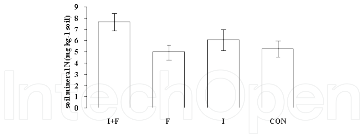
Figure 5. Soil mineral nitrogen in irrigation experiment, Kherson
