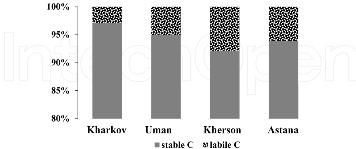
Figure 13. Distribution of labile and stable C in different Mollisols from four studied sites
